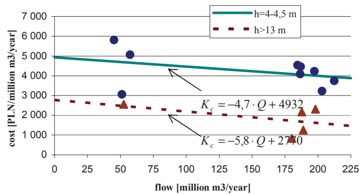
Figure 5. Relation between the unit annual cost per million m^3 /year of water flow and the unit stream flow as well as the water head Source: own research
