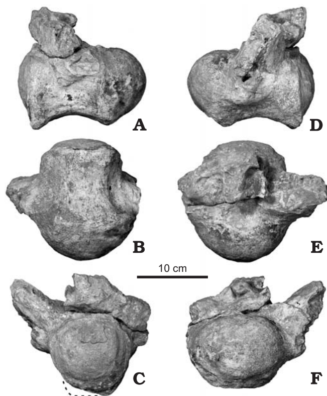
Fig. 5. Holotypic seventh sacral vertebra of the sauropod Neuquensaurus australis (Lydekker, 1893), MLP Ly 1, from the Late Cretaceous of Neuquén, Argentina in left lateral (A), ventral (B), anterior (C), right lateral (D), dorsal (E), and posterior (F) views.
