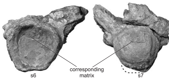
Fig. 1. Holotypic sacrum of the sauropod Neuquensaurus australis (Lydekker, 1893), MLP Ly 1 and 7, from the Late Cretaceous of Neuquén, Argentina. Posterior view of sixth sacral vertebra and anterior view of seventh sacral vertebra showing corresponding matrix, which snaps together when the vertebrae are articulated. The abbreviations (s6–s7) indicate sacral vertebral identity. Dashed lines indicate missing bone.
