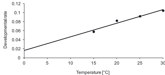
Fig. 1. Developmental rate for total immature developmental of S. maydis at different constant temperatures
