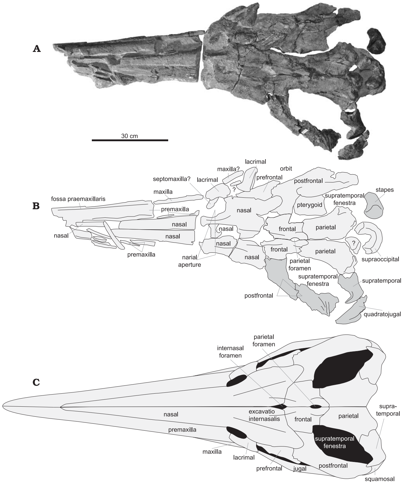
Fig. 2. Ophthalmosaurid ichthyosaur Platypterygius hercynicus Kuhn, 1946, MNHN 2010.4, from the late Albian of Saint-Jouin-Bruneval, France. Skull roof anatomy. A. Photograph. B. Explanatory drawing. The bones found in connection are coloured in pale grey and the bone placed manually at their supposed position are coloured in dark grey. C. Reconstruction. This reconstruction is designed to provide an overview of the skull roof of MNHN 2010.4; please refer to the description and the other figures for anatomical comparison or character state scoring in phylogenetic analysis. The anterior ramus of the nasal is developed, forming the dorsomedial part of the rostrum over a very long distance. The nasal is also developed posterolaterally, overlapping the postfrontal extensively. The frontal participates to three cranial openings: the internasal foramen anteriorly, the pineal foramen posteromedially, and the supratemporal fenestra posterolaterally.
