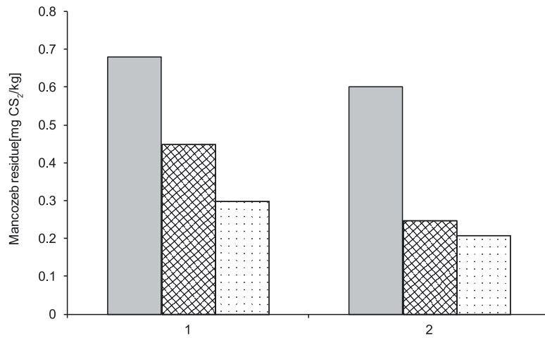
Fig. 2. Mancozeb residue reduction in blackcurrant fruit after washing with water, and aqueous ozone solution: grey – initial residue, grid – residue after water treatment, dots – residue after 0.5 h of treatment using 2 ppm ozone solution in water
