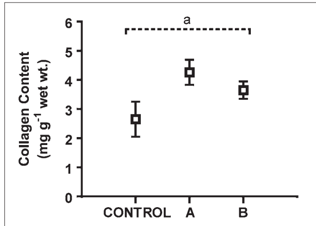
FIGURE 4 Total collagen content. Mouse aorta sections taken from the same samples used for elastic recoil measurements, were additionally analyzed for collagen content (mg g -1 wet wt.) using the approach described in the methods section. Each point represents the mean \pm SE. Significant differences between the means are given: a = P < 0.05 – Kruskal-Wallis (Nonparametric ANOVA). Animals allocated to the three groups were n = 6 for all.
