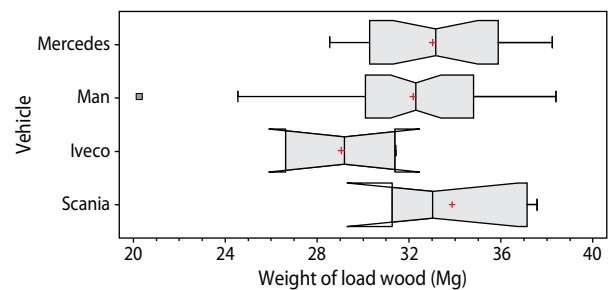
Fig. 6. Weights of single loads hauled by the analyzed sets
