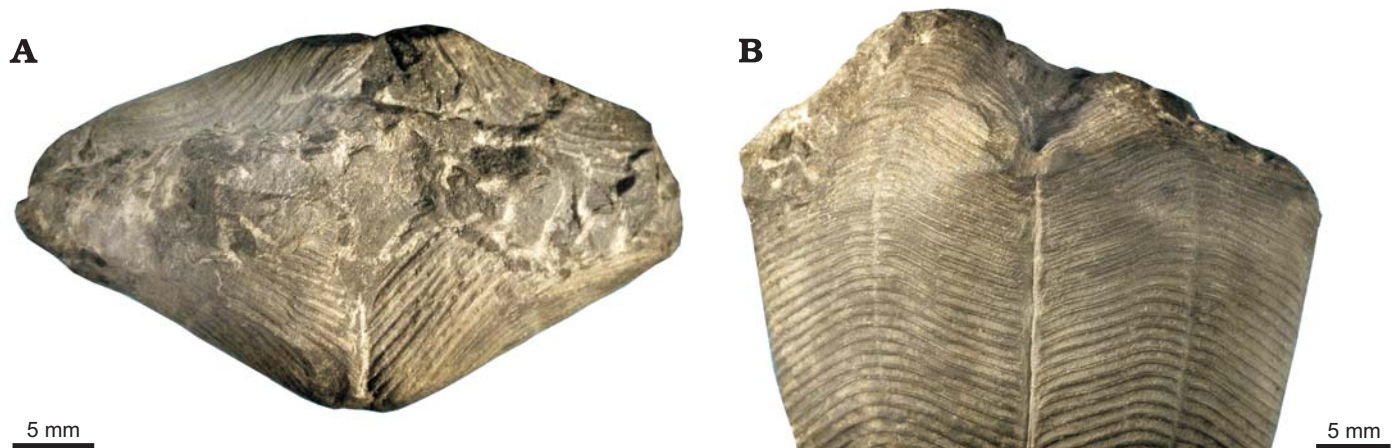
Fig. 4. Closure with triangular terminal ends in a toptype of Conularia brongniarti Archiac and Verneuil, 1842 from the Devonian of Néhou (Manche, France), FSL-EM 17501, in apertural ( A ) and lateral ( B ) views.
