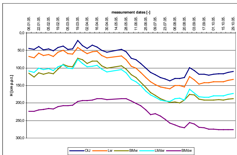
Figure 6. Ground water levels in different forest sites, the Marianka Forest Division, hydrological year 2005 [p.p.t. = under ground surface]
