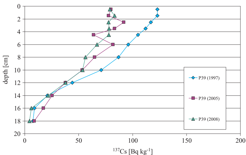
Figure 11. Vertical distribution of ^{137}\text{Cs} in sediments from the Bornholm Basin in 1997, 2005 and 2008 (measurement uncertainty 3–7%)
