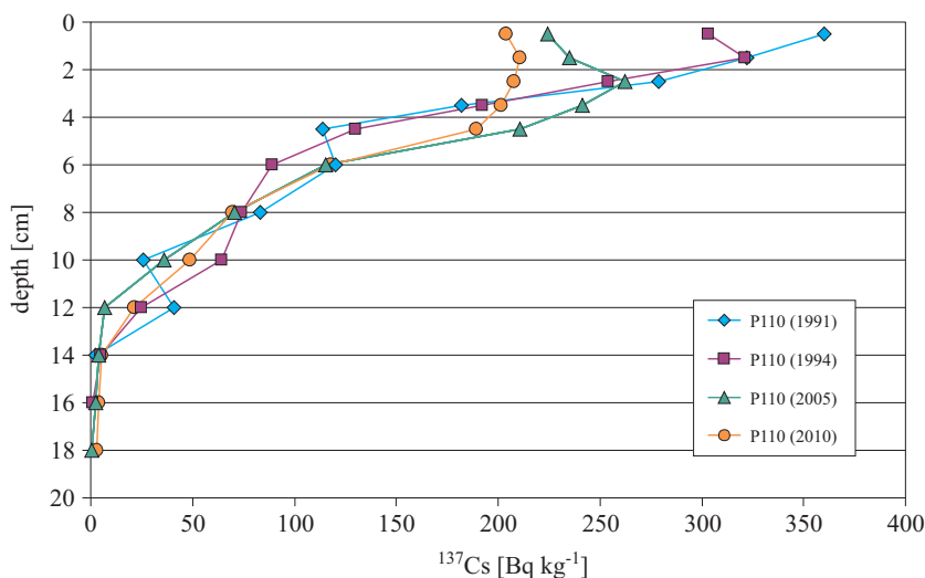
Figure 9. Vertical distribution of ^{137}\text{Cs} in sediments from the Gulf of Gdańsk in 1991, 1994, 2005 and 2010 (measurement uncertainty 3–7%)
