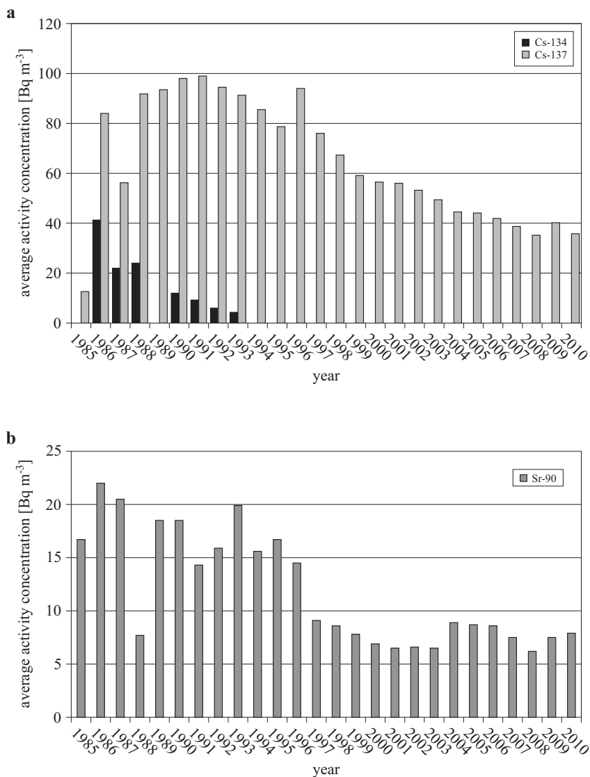
Figure 3. Changes in average activity concentrations of ^{134}\text{Cs} , ^{137}\text{Cs} (a) and ^{90}\text{Sr} (b) in seawater in the period 1985–2010 (data from 1985–1998 after Tomczak (1999), data from 1999–2010 after Zalewska & Saniewski (2012))
