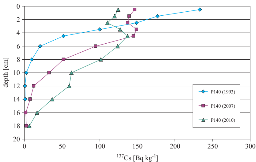
Figure 10. Vertical distribution of ^{137}\text{Cs} in sediments from the SE Gotland Basin in 1993, 2007 and 2010 (measurement uncertainty 3–7%)
