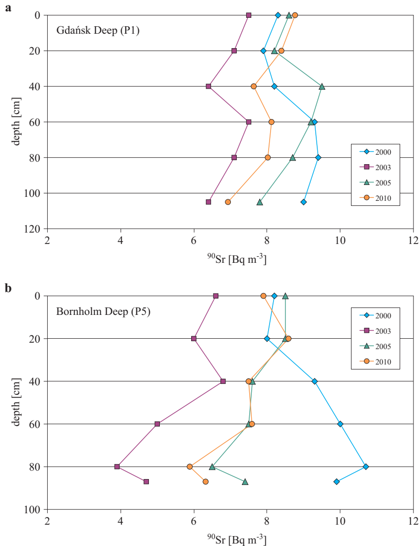
Figure 5. Vertical distribution of ^{90}\text{Sr} activity concentrations in the Bornholm and Gdańsk Deeps (measurement uncertainty 4–7%)
