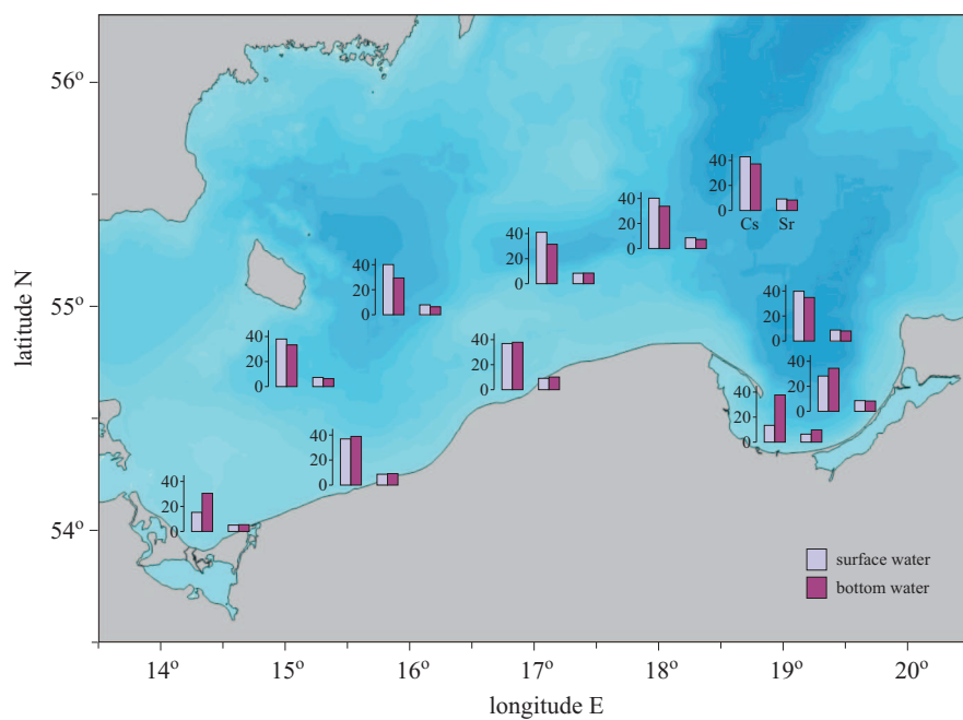
Figure 7. Activity concentrations of ^{137}\text{Cs} and ^{90}\text{Sr} in the surface and bottom waters of the southern Baltic Sea in 2010 (Zalewska & Saniewski 2012)
