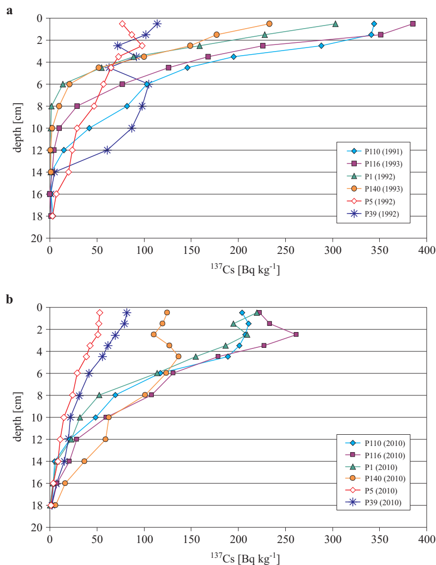
Figure 8. Vertical distribution of ^{137}\text{Cs} in marine sediments at six locations in the southern Baltic Sea in the early 1990s (a) and in 2010 (b) (measurement uncertainty 3–7%)
