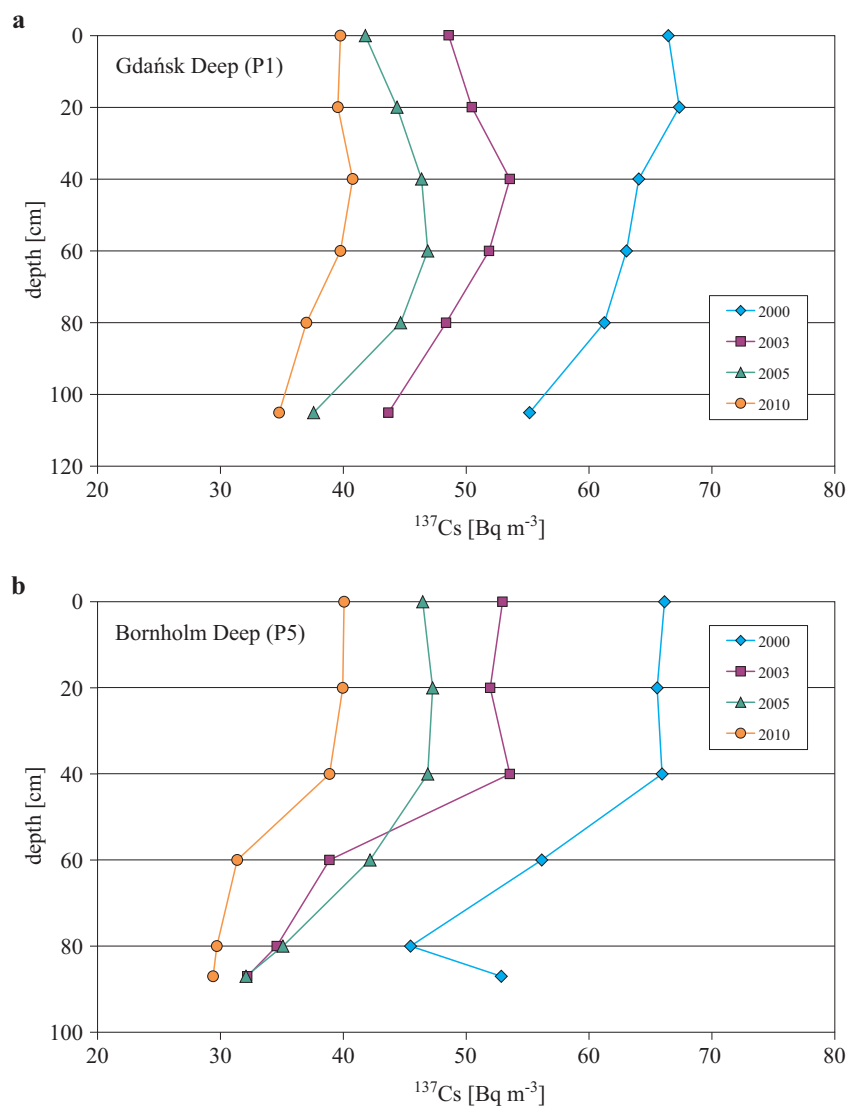
Figure 4. Vertical distribution of ^{137}\text{Cs} activity concentrations in the Bornholm and Gdańsk Deeps (measurement uncertainty 1.8–2.5%)
