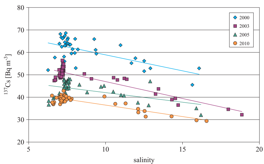
Figure 6. Relationships between activity concentrations of ^{137}\text{Cs} and salinity of Baltic Sea water
