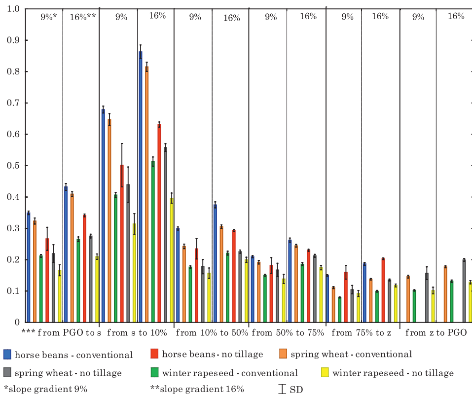
Fig. 2. Mean loss of magnesium ( \text{kg ha}^{-1} ) in different periods of crop management. Periods of management after SCHWERTMANN et al. (1987) – see Figure 1
