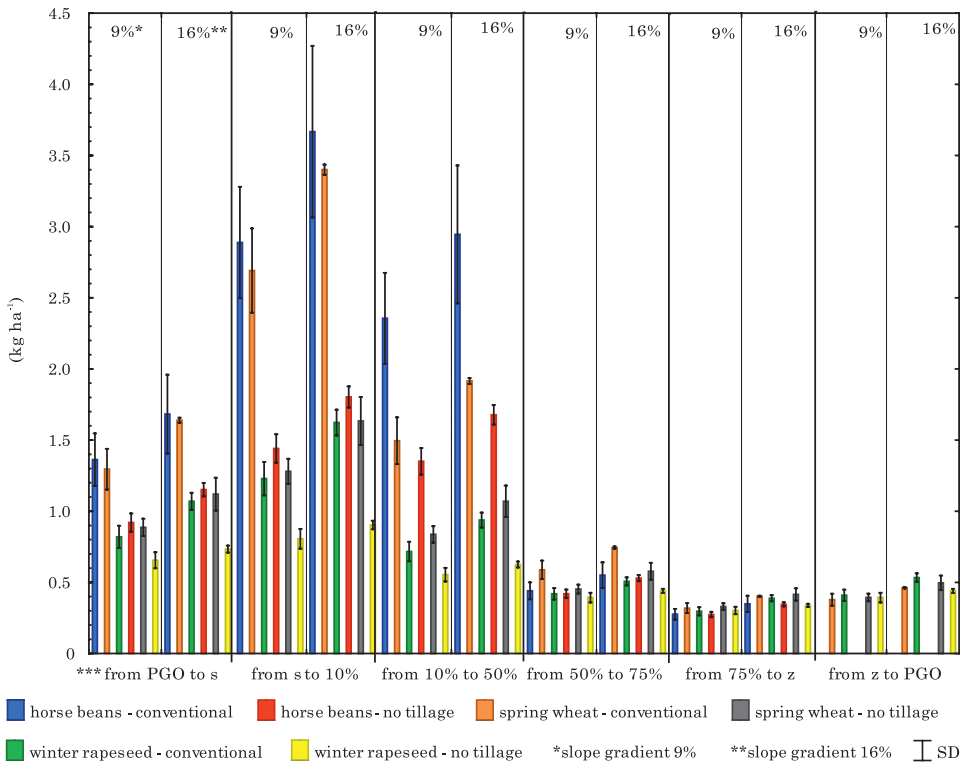
Fig. 1. Mean loss of calcium (kg ha -1 ) in different periods of crop management.
