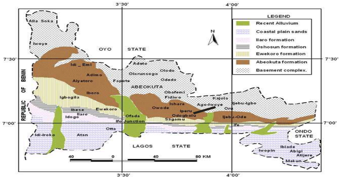
Figure 2.0: Geological map of Ogun State showing different areas (Adopted by Olurin et al. , 2012).
