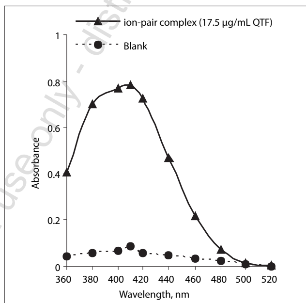
Figure 1 Absorption spectra of QTF-BPB ion-pair complex and blank.
