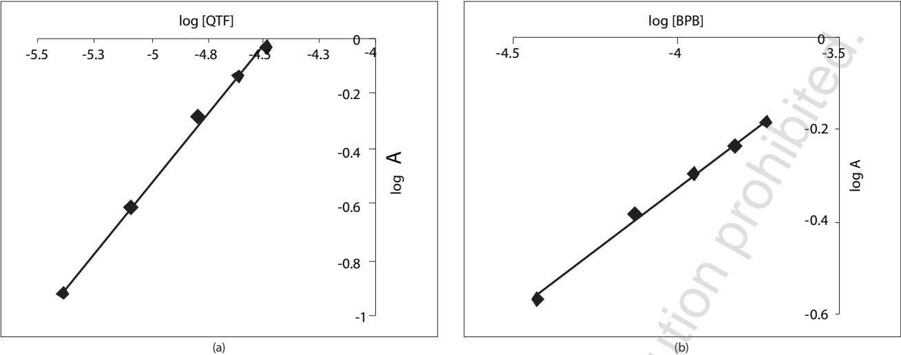
Figure 4 Limiting logarithmic plots to evaluate the stoichiometry of QTF-BPB ion-pair complex in method A: (a) variation of [QTF] and (b) variation [BPB].
