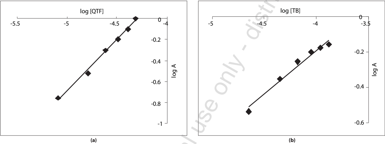
Figure 5 Limiting logarithmic plots to evaluate the stoichiometry of QTF-TB ion-pair complex in method B: (a) variation of [QTF] and (b) variation [TB].
