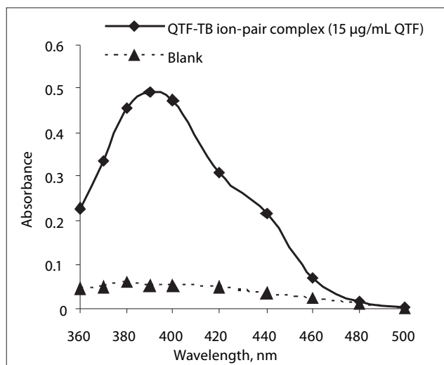
Figure 2 Absorption spectra of QTF-TB ion-pair complex and blank.
