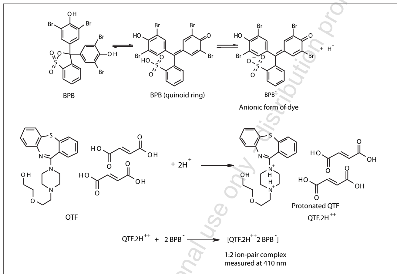
Scheme 1 Possible reaction pathway for the formation of QTF-BPB ion-pair complex.
