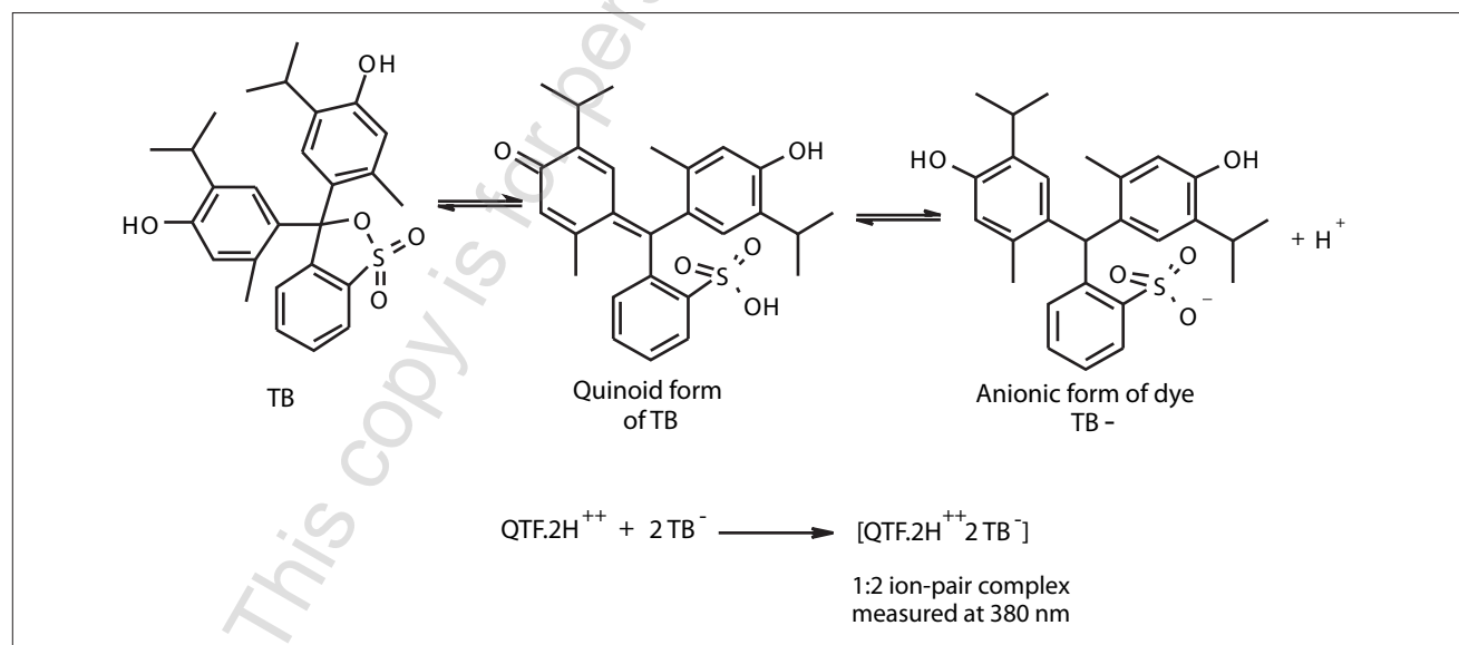
Scheme 2 Possible reaction schemes for the formation of QTF-TB ion-pair complex.
