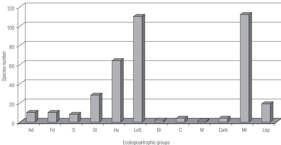
Fig. 2. Arrangement of fungal species in ecological-trophic groups.
