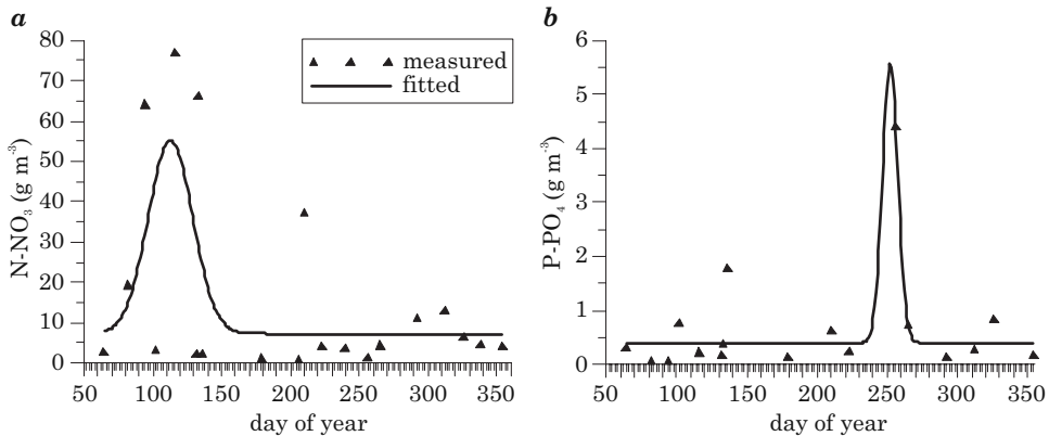
Fig. 6. Nitrate nitrogen (a) and phosphate (b) concentration versus day of the year
