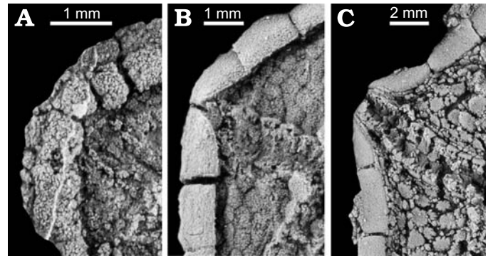
Fig. 8. Ontogenetic development of marginal ring and ambulacral tips in edrioasteroid echinoderm Cambraster cannati Miquel (1894) from early juveniles (A), late juveniles (B), and adult (C) specimens. The three photographs represent ambulacrum E.
