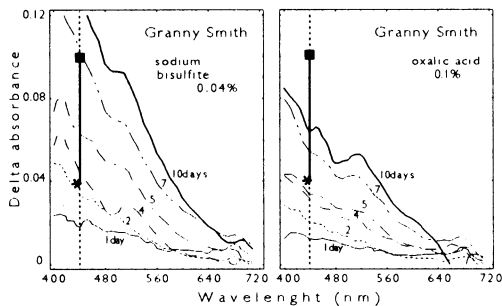
Fig. 2. An example of a storage related pattern of the absorbance difference spectra of apple slices in c.v. Granny Smith cut at different concentrations in either sodium bisulfite or oxalic acid. The line indicates the interval from a visually detectable '*' until the acceptable level of browning '■'.
