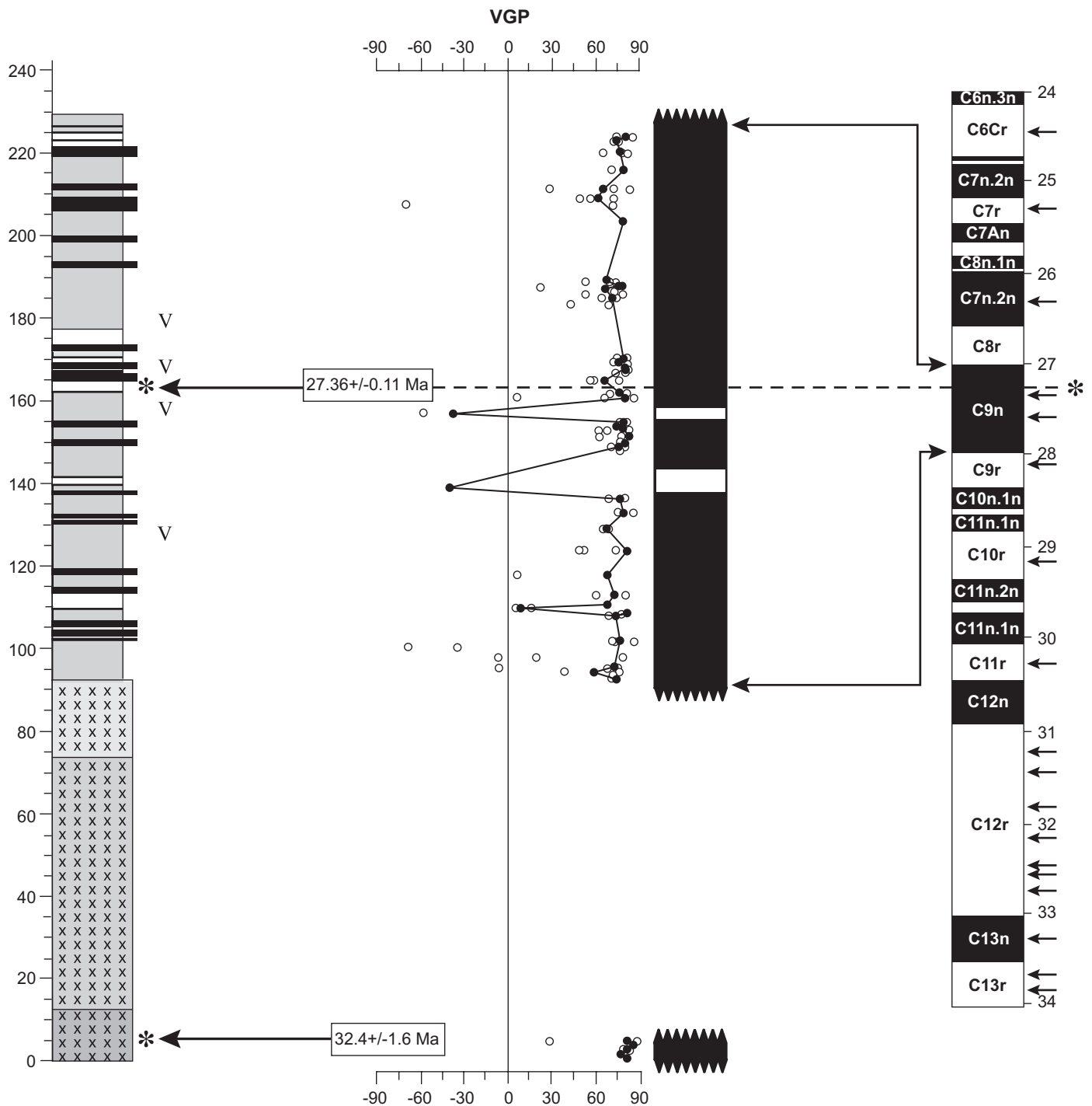
Fig. 2. Diagram of the Chilga stratigraphic section. The section has more than 90 m of volcanics at its base that are overlain by at least 130 m of fluvial and alluvial sediments. Stepwise alternating-field demagnetization was carried out on 118 samples with generally three samples per stratigraphic level. Paleomagnetic reversal stratigraphy demonstrates a dominance of normal polarity, and an ^{40}\text{Ar}/^{39}\text{Ar} age of 27.36 \pm 0.11 Ma for a tuff in the upper portion of the sedimentary sequence at about 165 m provides an absolute tie point to Chron C9n (27.946–27.004 Ma). Small arrows to the far right of the geomagnetic polarity time scale of Cande and Kent (1995) represent “tiny wiggles,” and the two brief reversal events within Chron 9 may be present at Chilga, providing additional but more indirect support for this correlation. Together these data suggest that this section is probably limited to the duration of this Chron (<1 Myr). Vertebrate-bearing horizons (V) occur primarily through the middle part of the section.
