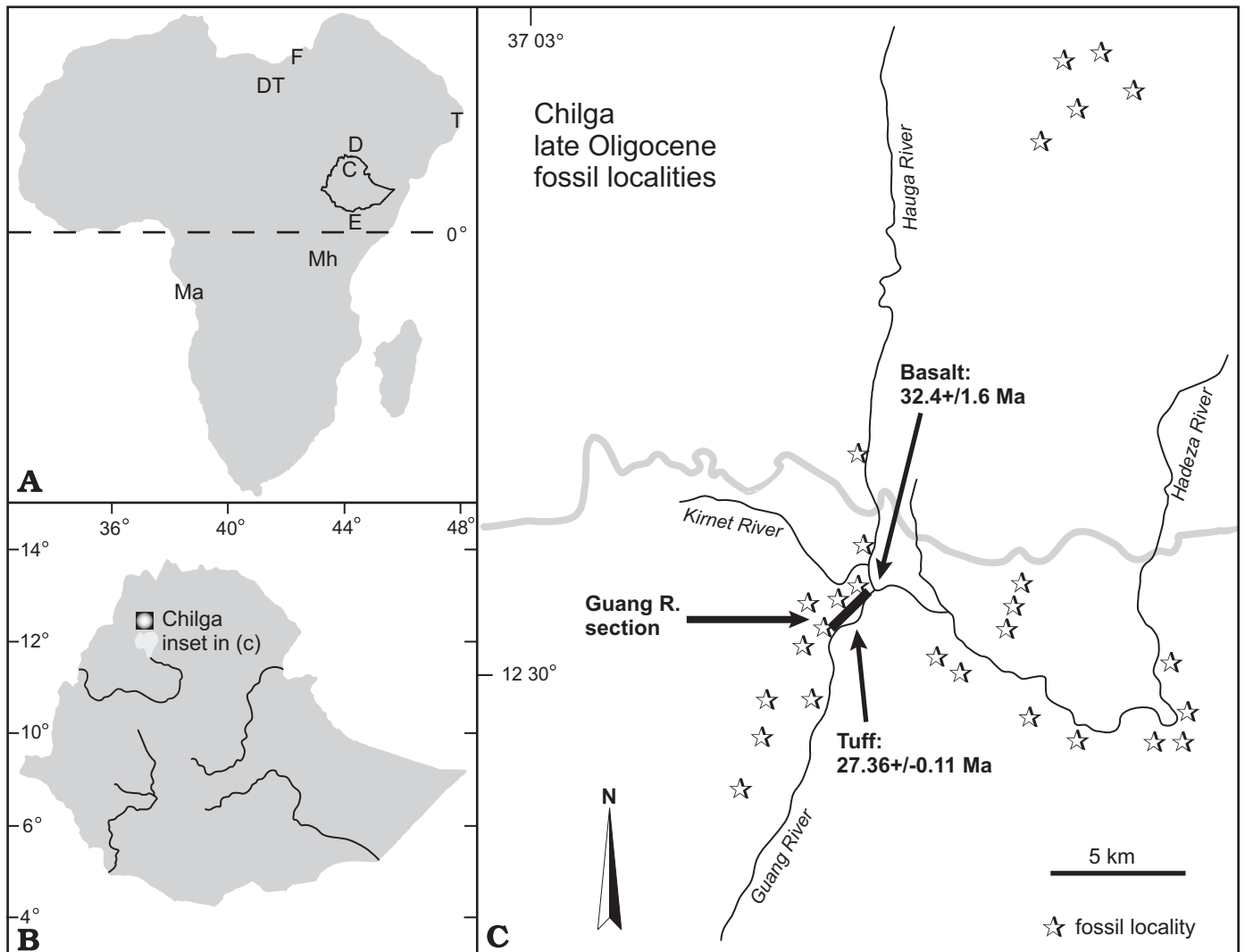
Fig. 1. A. Map of Afro-Arabia with several important Paleogene terrestrial mammal sites (underlined characters denote abbreviations for the localities marked on the map), including C hilga (Ethiopia), D ogali (Eritrea), Lothidok ( E ragaleit Beds, Kenya), F ayum (Egypt), D or el T alha (Libya), M alembe (Angola), M ahenge (Tanzania), and T haytini and T aqah (Oman). Outline of Ethiopia is inset. B. Map of Ethiopia showing the location of Chilga, north of Lake Tana. C. Detailed map of the Chilga area showing the fossil localities, geologic section (Fig. 2), and dated rock sample localities, along the Guang and Hauga Rivers.
