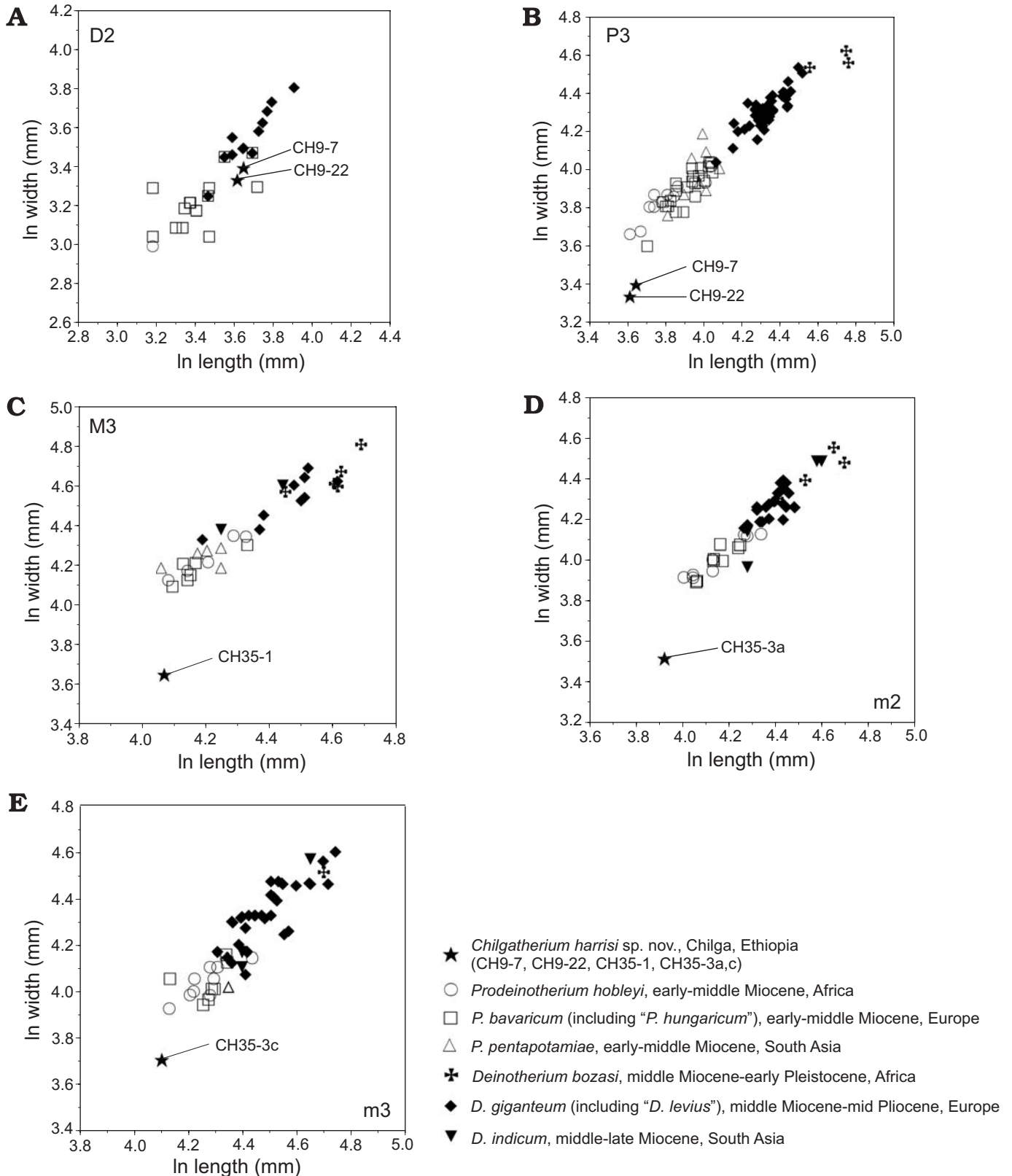
Fig. 6. Bivariate plots of natural log-transformed crown length versus width of selected cheek teeth in Chilgatherium harrisi sp. nov. and other deinotheres species. Comparative dimensions are from Bachmann (1875), Weinsheimer (1883), Roger (1886), Andrews (1911), Cooper (1922), Palmer (1924), Éhik (1930), MacInnes (1942), Gräf (1957), Sahni and Tripathi (1957), Symeonidis (1970), Harris (1973, 1977, 1983, 1987), Gaziry (1976), Tobien (1988), Tsoukala and Melentis (1994), Huttunen (pers. com.; 2000), Sach and Heizmann (2001), and Sanders (2003). A. Specimens CH9-7 and CH9-22 compared with D2 in other deinotheres. Note that in this comparison, the Chilga specimens appear anomalously large, relative to size contrasts between other cheek teeth from the Chilga deinotheres sample and those of Prodeinotherium and Deinotherium . B. P3. C. M3. D. m2. E. m3.
