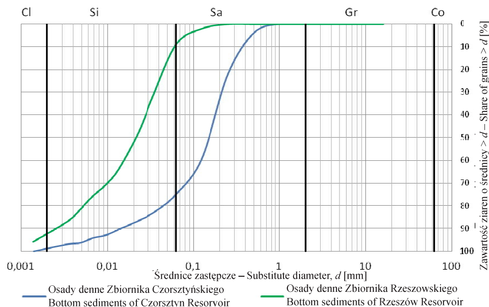
RYSUNEK 1. Krzywe uziarnienia badanych osadów dennych FIGURE 1. Grain size distribution curves of the tested bottom sediments
