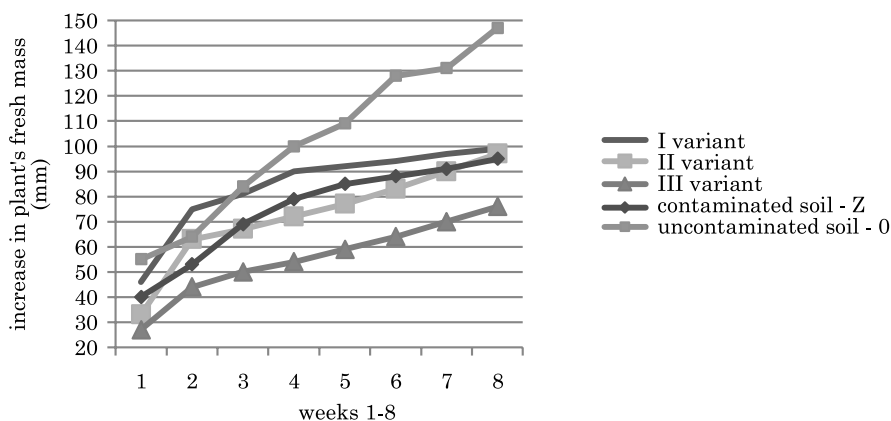
Fig. 1. Growth rate of common orchardgrass fresh mass in the pot cultivation
