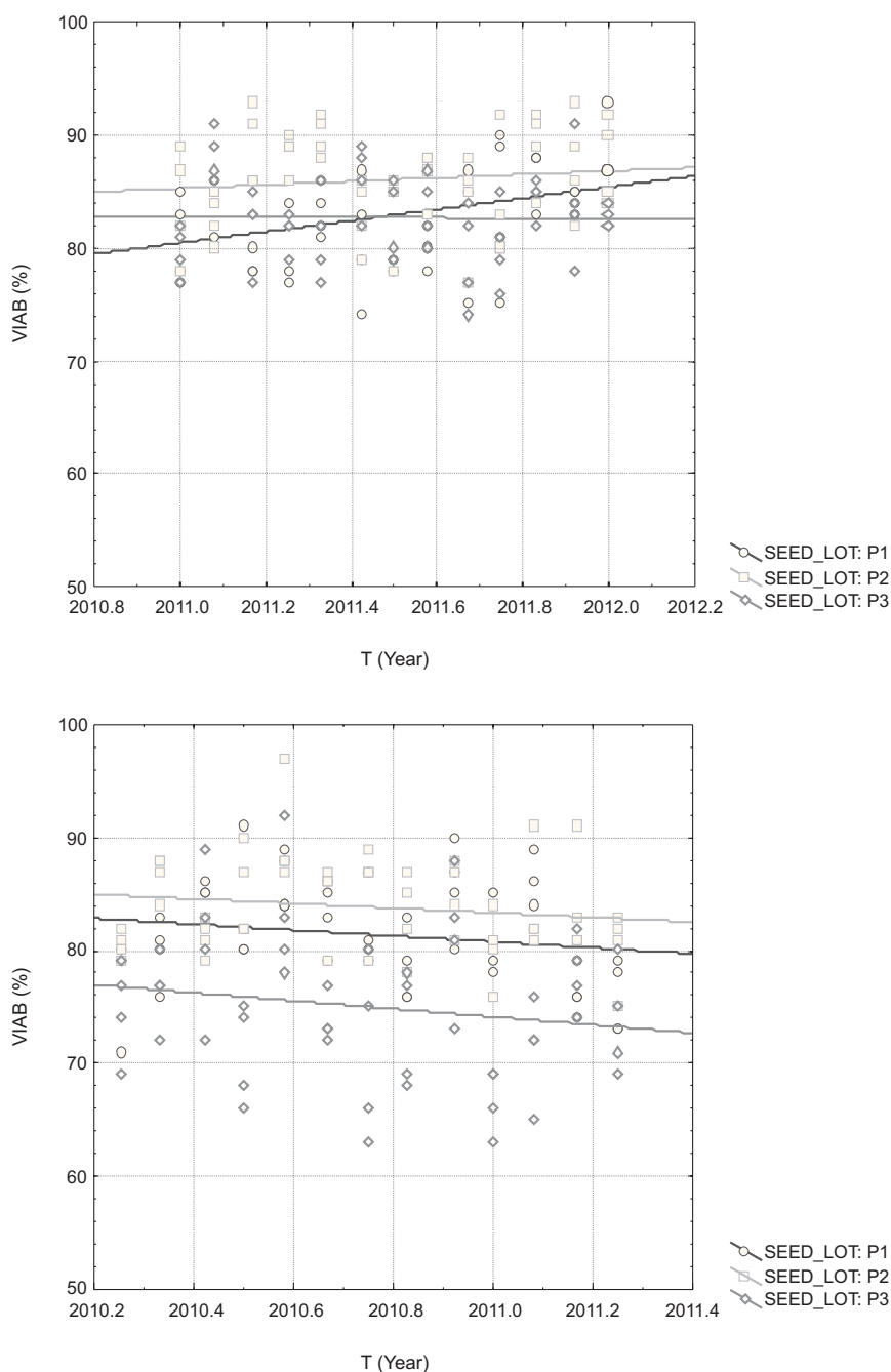
Fig. 7. Basic trends in European beech ( Fagus sylvatica ) seed viability (VIAB; in per-cent) against time (T) using the least sum-of-square method: the seed lot P1: VIAB = -9861.7 + 4.9439 \cdot T , r = 0.360 , p = 0.0089 ; P2: VIAB = -2999.8 + 1.5341 \cdot T , r = 0.116 , p = 0.41 ; P3: VIAB = 543.4 - 0.2290 \cdot T , r = -0.019 , p = 0.89 ; 5102: VIAB = 5310.0 - 2.6003 \cdot T , r = -0.178 , p = 0.21 ; 7208: VIAB = 4200.8 - 2.0475 \cdot T , r = -0.153 , p = 0.28 ; 7209: VIAB = 7201.2 - 3.5441 \cdot T , r = -0.173 , p = 0.22
