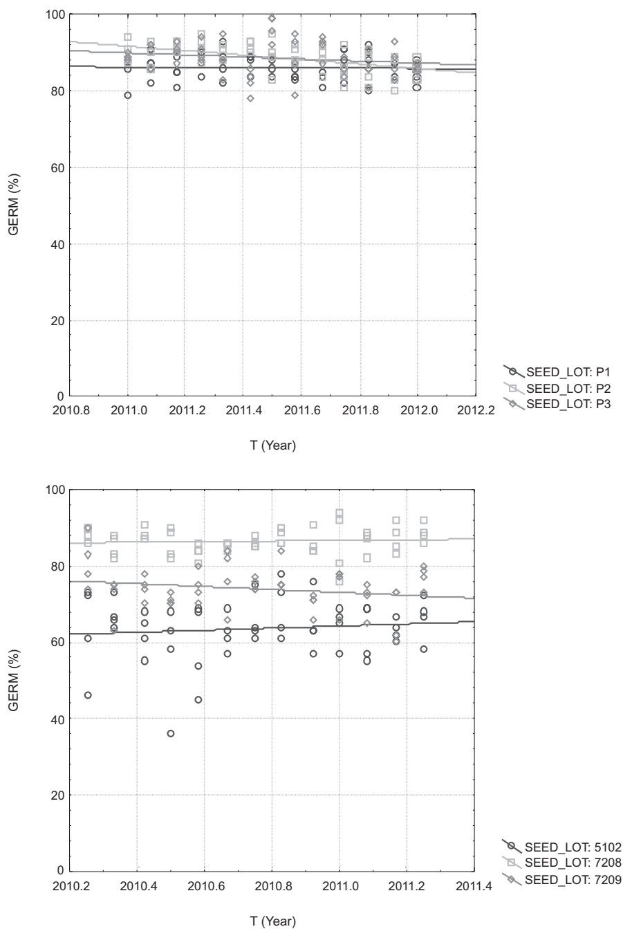
Fig. 1. Basic trends in European beech ( Fagus sylvatica ) seed germination (GERM; in per-cent) against time (T) using the least sum-of-square method: the seed lot P1: \text{GERM} = 832.7 - 0.3712 \times T , r = -0.036 , p = 0.80 ; P2: \text{GERM} = 11828.7 - 5.8364 \times T , r = -0.488 , p = 0.0002 ; P3: \text{GERM} = 5450.2 - 2.6655 \times T , r = -0.185 , p = 0.19 ; 5102: \text{GERM} = -5466.7 + 2.7504 \times T , r = 0.111 , p = 0.43 ; 7208: \text{GERM} = -1489.6 + 0.7838 \times T , r = 0.072 , p = 0.61 ; 7209: \text{GERM} = 7684.6 - 3.7849 \times T , r = -0.210 , p = 0.13
