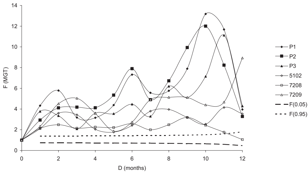
Fig. 5. Ratio of semi-variances to variance ( F ) plotted against time-distance ( D ) for mean germination time (MGT) of European beech ( Fagus sylvatica ) seed lots. The bold curve shows an example of a significant periodicity (P2)
