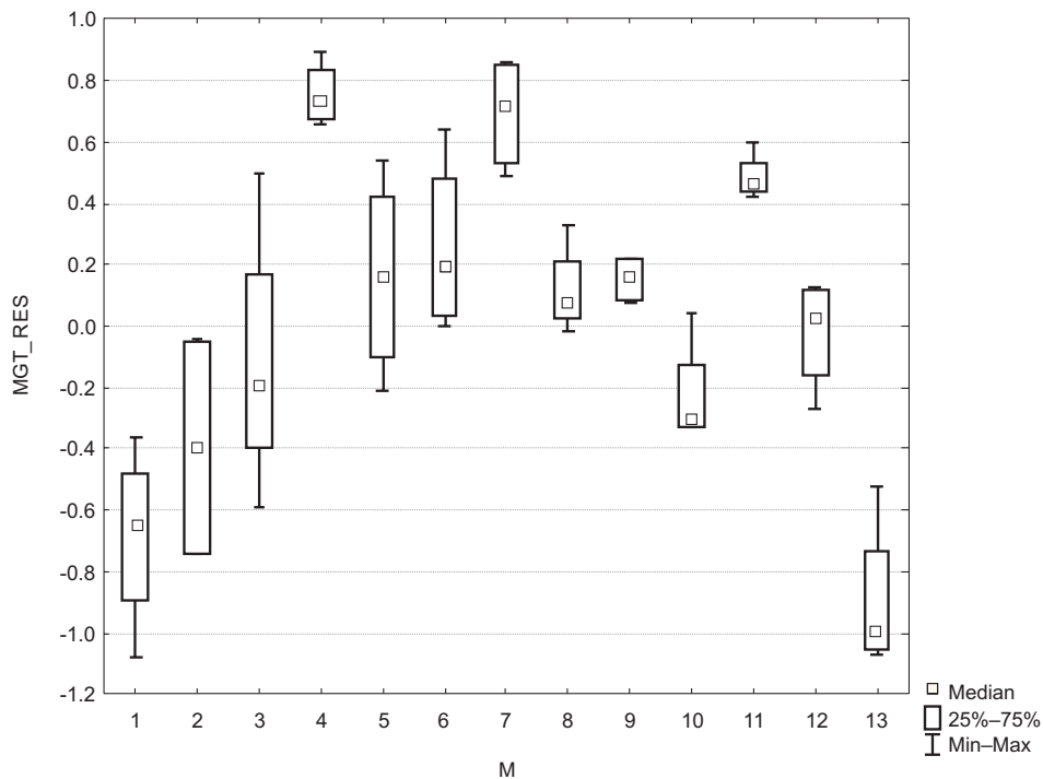
Fig. 6. Residuals of mean germination time (MGT_RES; in weeks) to linear regression of the European beech ( Fagus sylvatica ) seed lot P2 which shows a significant periodicity (compare with Fig. 5). M – number of months of the analyses (1 = January 2011; 13 = January 2012)
