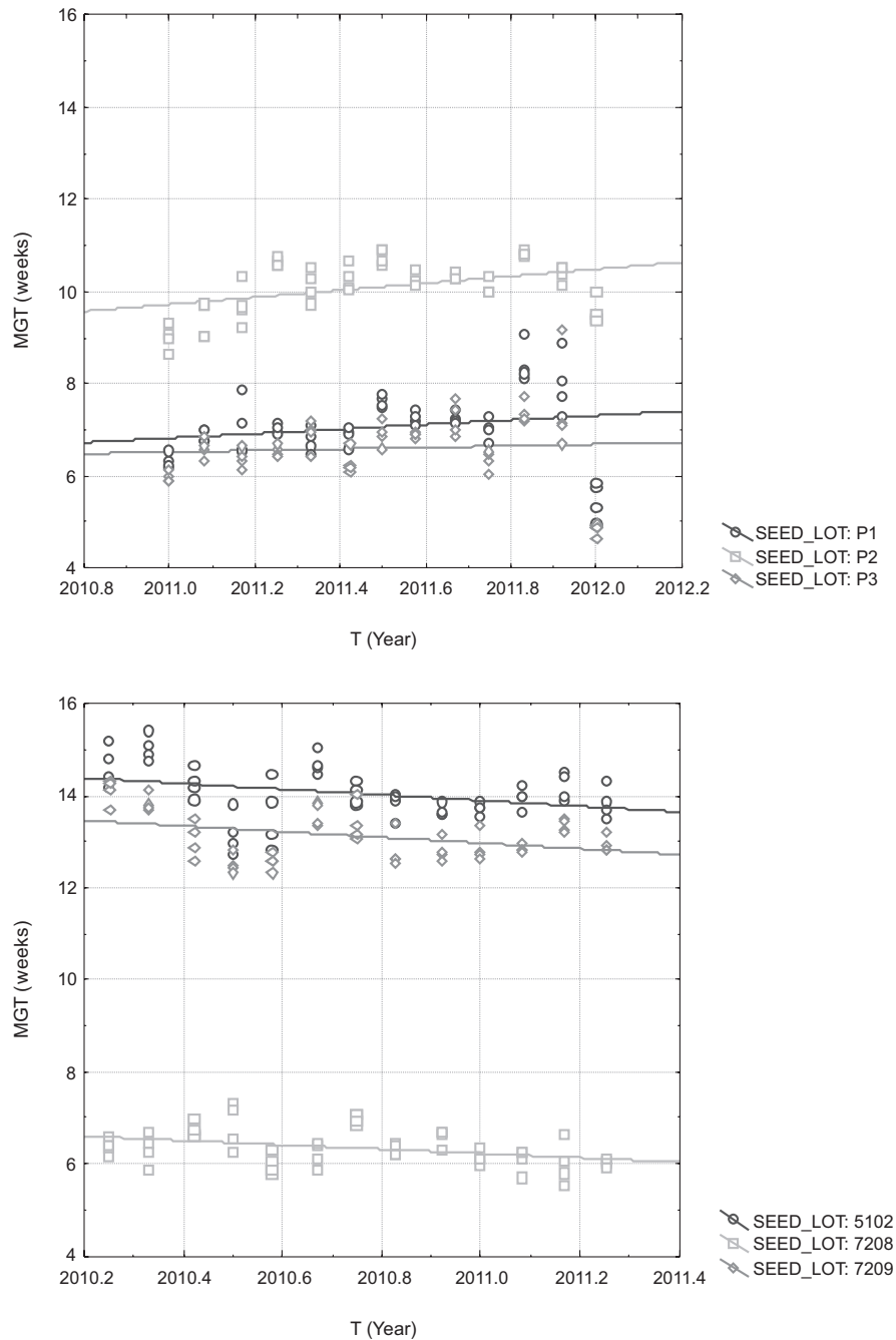
Fig. 4. Basic trends in European beech ( Fagus sylvatica ) seed mean germination time (MGT; in weeks) against time (T) using the least sum-of-square method: the seed lot P1: MGT = -976.88 + 0.4892 \times T , r = 0.200 , p = 0.15 ; P2: MGT = -1521.67 + 0.7615 \times T , r = 0.415 , p = 0.0022 ; P3: MGT = -333.40 + 0.1690 \times T , r = 0.071 , p = 0.62 ; 5102: MGT = 1250.72 - 0.6150 \times T , r = -0.331 , p = 0.016 ; 7208: MGT = 943.83 - 0.4662 \times T , r = -0.361 , p = 0.0085 ; 7209: MGT = 1256.86 - 0.6185 \times T , r = -0.359 , p = 0.0089
