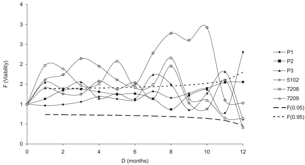
Fig. 8. Ratio of semi-variances to variance (F) plotted against time-distance (D) for viability of European beech ( Fagus sylvatica ) seed lots. The bold curve shows an example of a significant periodicity (lot 5102)
