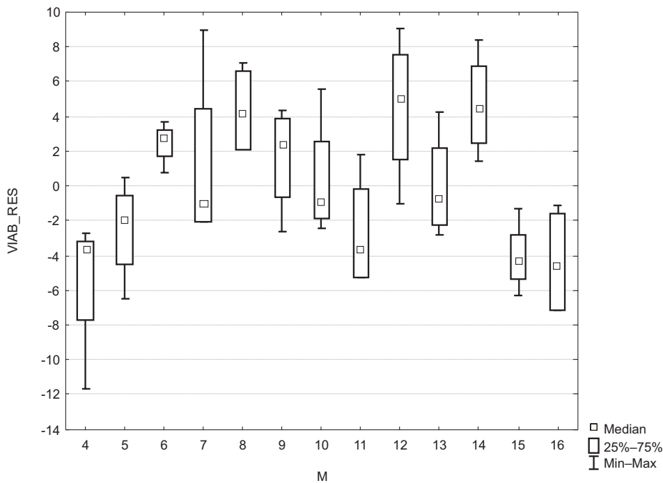
Fig. 9. Residuals of viability (VIAB_RES; in percent) to linear regression of the European beech ( Fagus sylvatica ) seed lot 5102 which shows a significant periodicity (compare with Fig. 8). M –number of months of the analyses (4= April 2010, 16= April 2011)
