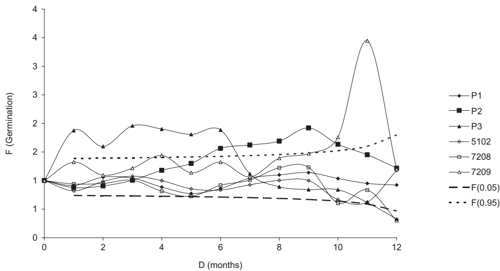
Fig. 2. Ratio of semi-variances to variance (F) plotted against time-distance (D) for germination of European beech ( Fagus sylvatica ) seeds by lots. The bold curve shows an example of a significant periodicity (lot P2)
