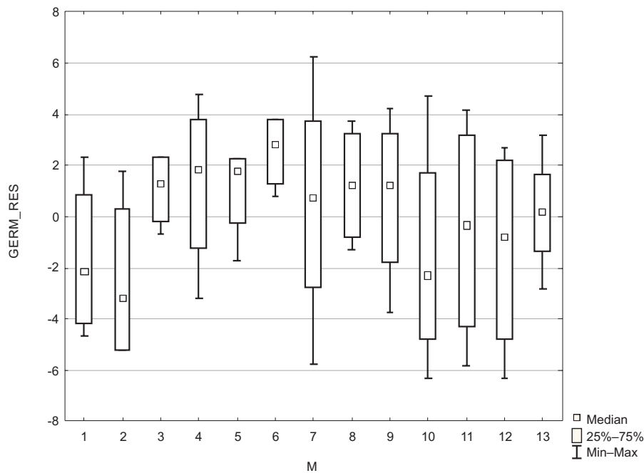
Fig. 3. Residuals of germination (GERM_RES; in per-cent) to linear regression of the European beech ( Fagus sylvatica ) seed lot P2 which shows a significant periodicity (compare with Fig. 2). M – number of months of the analyses (1 = January 2011; 13 = January 2012)
