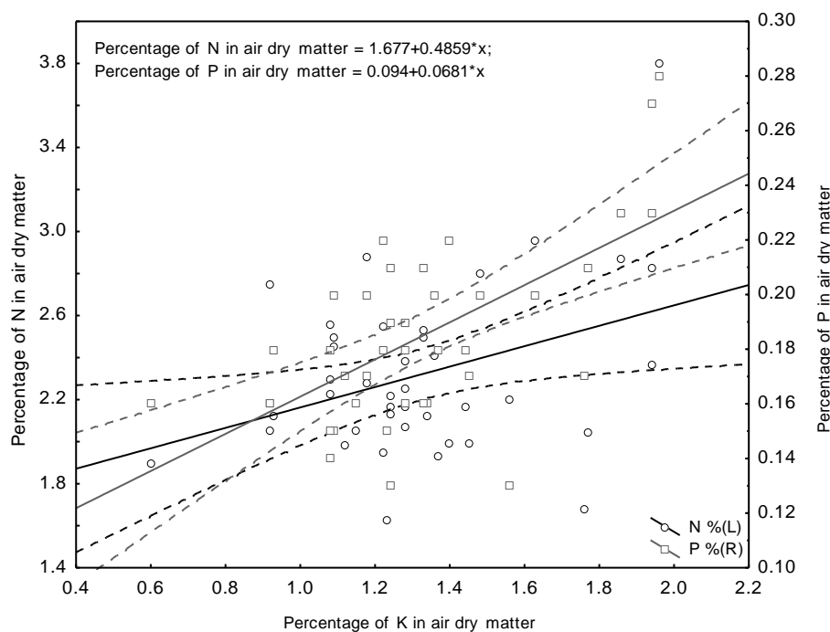
Fig. 1. Content of nitrogen (%N d.m.) and phosphorus (%P d.m.) in leaves of apple trees in relation to the level of potassium (%K d.m.) in that plant part
