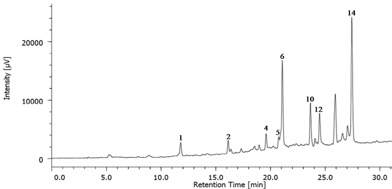
Figure 2. Chromatogram of phenolic standard mixture at 254 nm (A) and chromatogram of bound phenolic extract of Q. salicina leaves (B)
