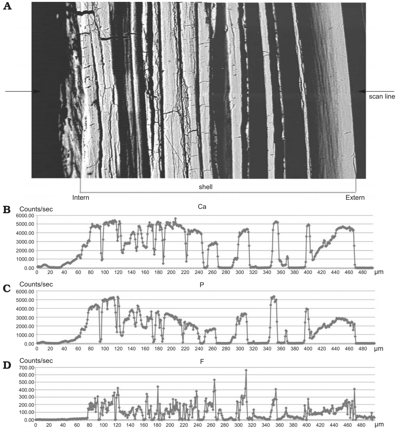
Fig. 8. Microprobe WDS scan line of Recent lingulid brachiopod Lingula anatina Lamark, 1801 (AF JL.An.Tra) from Japan. A . Shell section, the length of the portion measured is about 500 \mu\text{m} , and has been taken below the median adductor muscle. Ca ( B ), P ( C ), and F ( D ) are plotted according to the procedure described in the material and methods section and are concordant with fluorapatite mineral.
