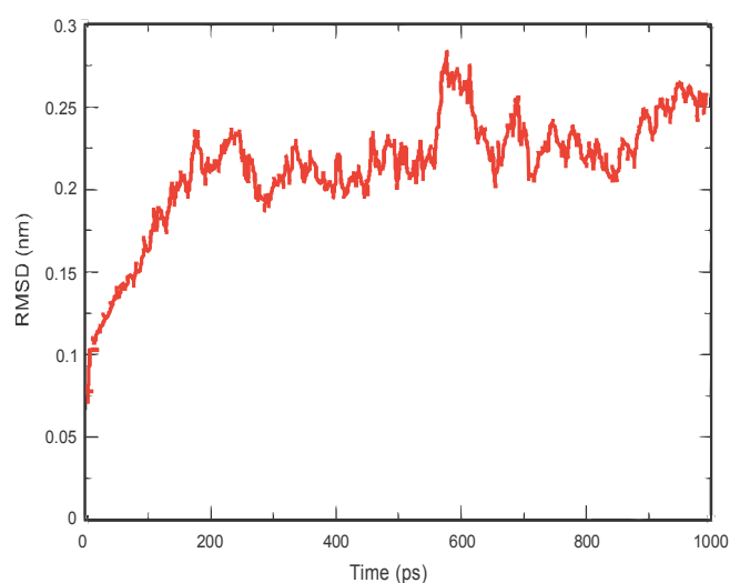
Fig. 5. Trajectories of the overall backbone (RMSD) of Actin-1 protein structure of Arabidopsis thaliana . The x-axis represents the simulation time in picoseconds. The y-axis represents RMSD in nm unit
