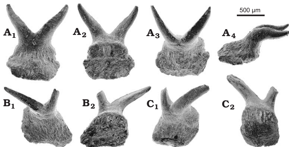
Fig. 3. Juvenile morphotype of the teeth of omalodontid shark Portalodus manoliniae sp. nov. from the Givetian of the Cairo quarry, New York, USA. A. NYSM 17736, paratype, in labial ( A_1 ), lingual ( A_2 ), occlusal ( A_3 ), and lateral ( A_4 ) views. B. NYSM 17756, in occlusal ( B_1 ) and lingual ( B_2 ) views. C. NYSM 17752, in occlusal ( C_1 ) and lingual ( C_2 ) views.
