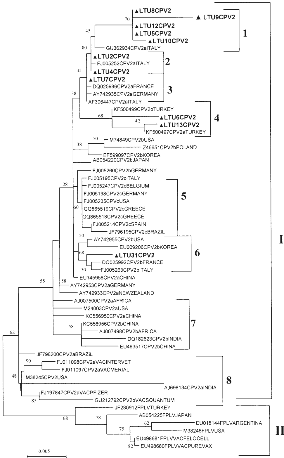
Fig. 1. The Maximum Likelihood phylogenetic tree of CPV VP2-coding (675 bp) region showing the relationships among 58 isolates of CPV. The tree with the highest log likelihood (-7330.6468) is shown. Lithuanian CPV isolates (n=11) VP2-sequences are presented in ▲Bold . Evolutionary analysis was conducted in MEGA6 (Tamura et al. 2013).
