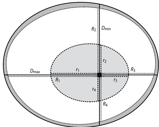
Figure 1. Method of measuring of log top end: D_{\max} – the bigger centric diameter with bark, D_{\min} – perpendicular (smaller) centric diameter with bark, R_n – outer radius of sapwood in n -direction, r_n – radius of heartwood in n -direction
