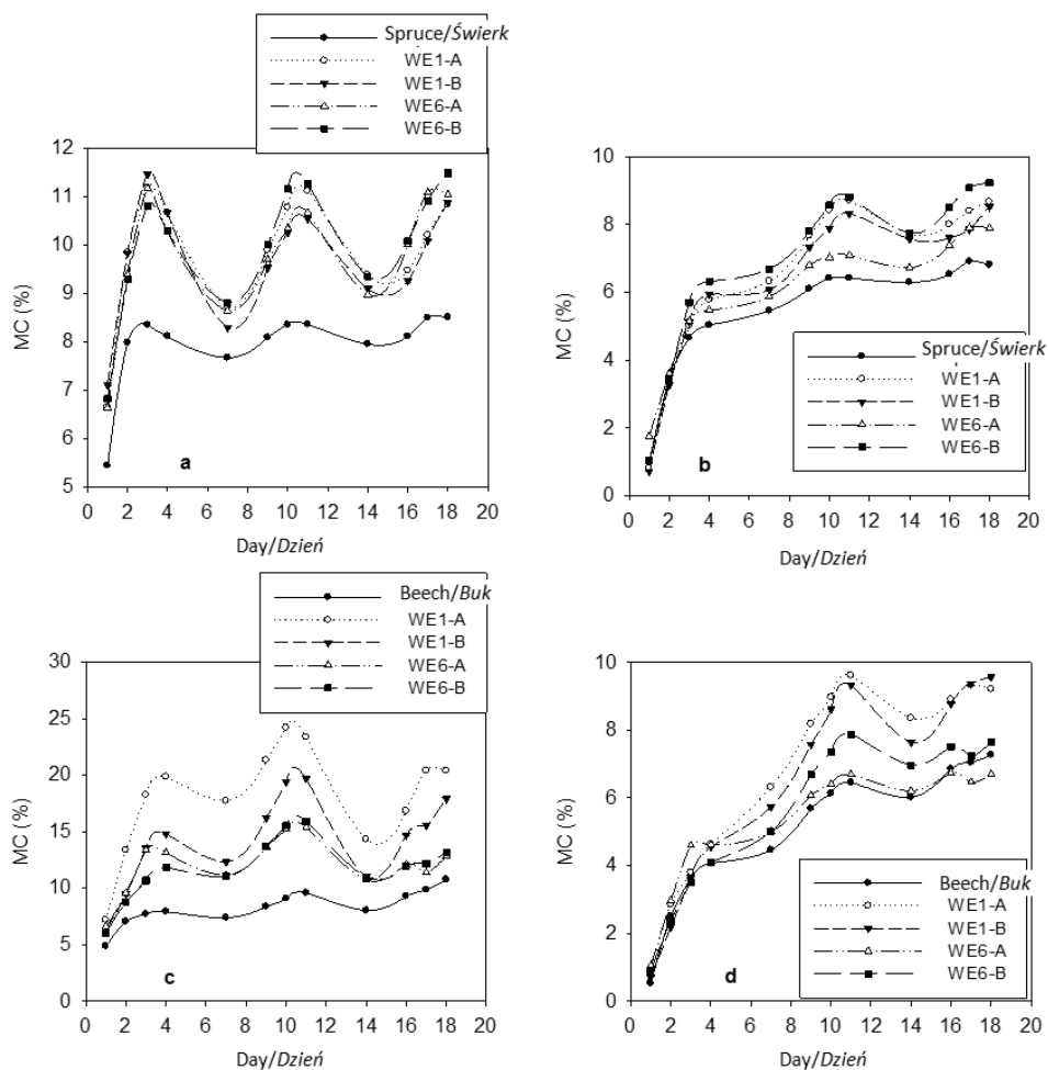
Fig. 4. Moisture content of polyethylene wax emulsion treated: (a) vacuum dried spruce, (b) spruce cured at 140 °C, (c) vacuum dried beech, and (d) beech cured at 140°C, before 10 minute non-continuous dipping in water
