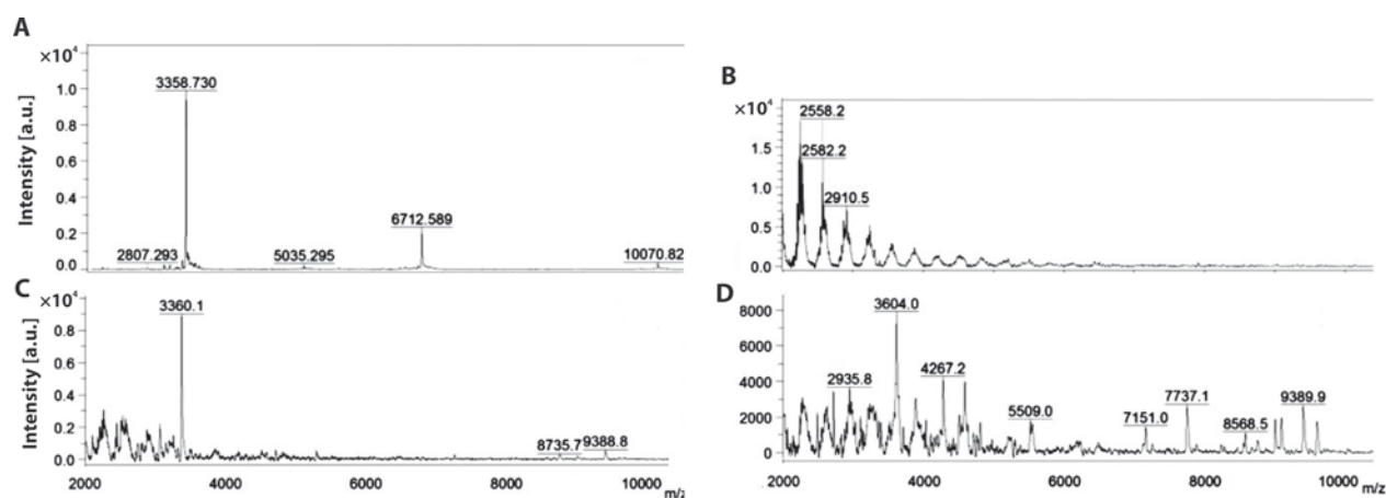
Fig. 1. Peak diagram of the substances found in homogenate samples of tissues from individual gypsy moth larvae after contact treatment with oligoRIBO-11 fragment (0.9 nmol · larva -1 ): A – standard oligoRIBO-11 fragment (3358.73 ± 10 Da); B – control; C, D – 30 and 60 min after the drop containing the oligoRIBO-11 fragment has dried, respectively. Analysis of all samples was carried out after 7 consistent washes of the larvae with a solution of water and 70% alcohol. The experiment was carried out three times. Diagrams detailing the characteristics of the groups are presented for each group in the experiment. Samples were pre-desalted on Illustra™ NAP™ -5 G-25 Sephadex™ columns according to manufacturer's instructions (GE Healthcare Life Sciences, USA) and then concentrated
