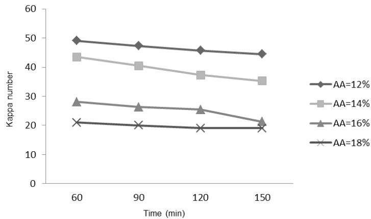
Fig. 3. Effect of cooking time at different AA charge on the kappa number of bamboo kraft pulps
