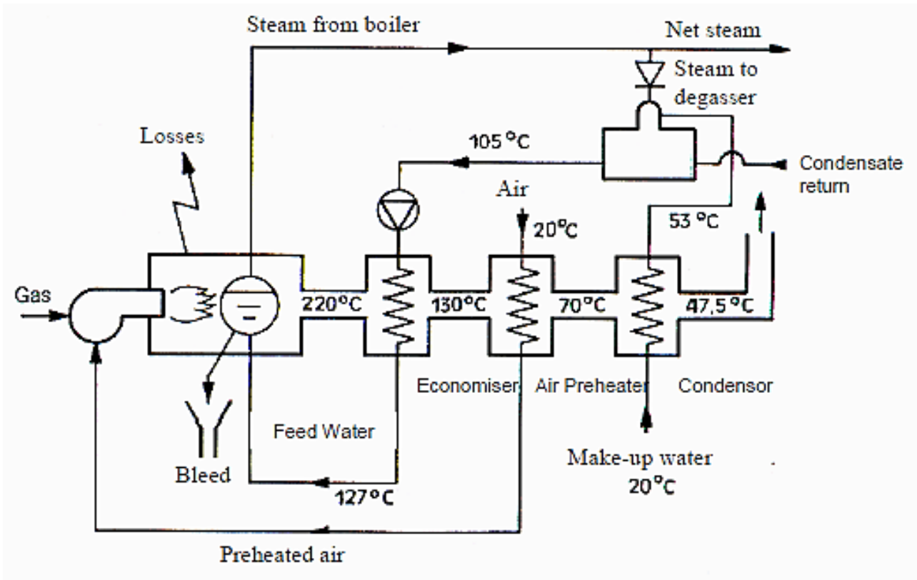
Figure 5. Production of steam from the boiler.
