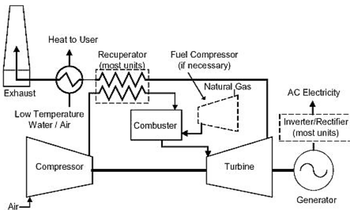
Figure 3. Micro-gas-turbine for electricity generation.
