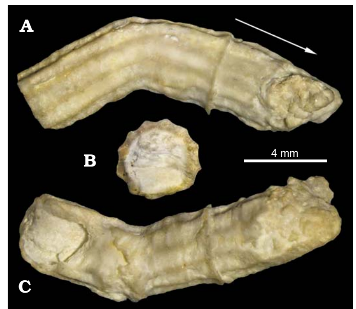
Fig. 3. The alleged serpulid Palaeotubus sosisensis gen. et sp. nov., holotype (MSNC 4499) from Pietra di Salomone limestone, Palazzo Adriano (Sicani Mountains, W Sicily); Wordian to upper Permian. The specimen was accurately cleaned from the rock but the white limestone is still visible infilling the tube lumen. Two opposite side views (A, C), growth direction arrowed, cross section (B).
