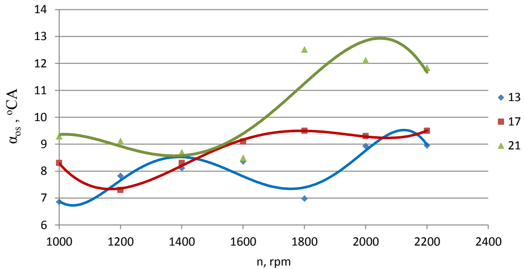
Fig. 5. Change to \alpha_{os} angle of self-ignition delay under the engine operating according to an external speed characteristic for three fuel angles of injection \alpha_{wv} = 13, 17 and 21 crankshaft rotation degrees
