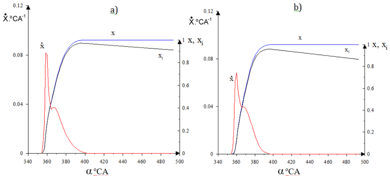
Fig. 6. Characteristics for relative heat emission during a combustion process x(\alpha) , x_i(\alpha) and \dot{x}(\alpha) under the engine operating at the factory set angle of injection \alpha_{wv} = 17 crankshaft rotation degrees and operating according to an external speed characteristic with a) n=1400 rpm and b) n=2000 rpm and fuelled by diesel
