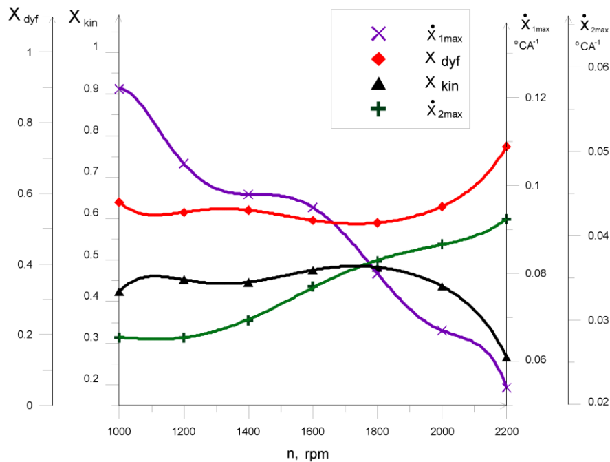
Fig. 9. Combustion process parameters for engine operation according to an external speed characteristic and angle of injection \alpha_{ww} = 21 crankshaft rotation degrees, where: x_{kin} – proportion of kinetic model combustion, x_{dyf} – proportion of diffusion model combustion, \dot{x}_{1max} and \dot{x}_{2max} – first and second maximum heat emission rate
