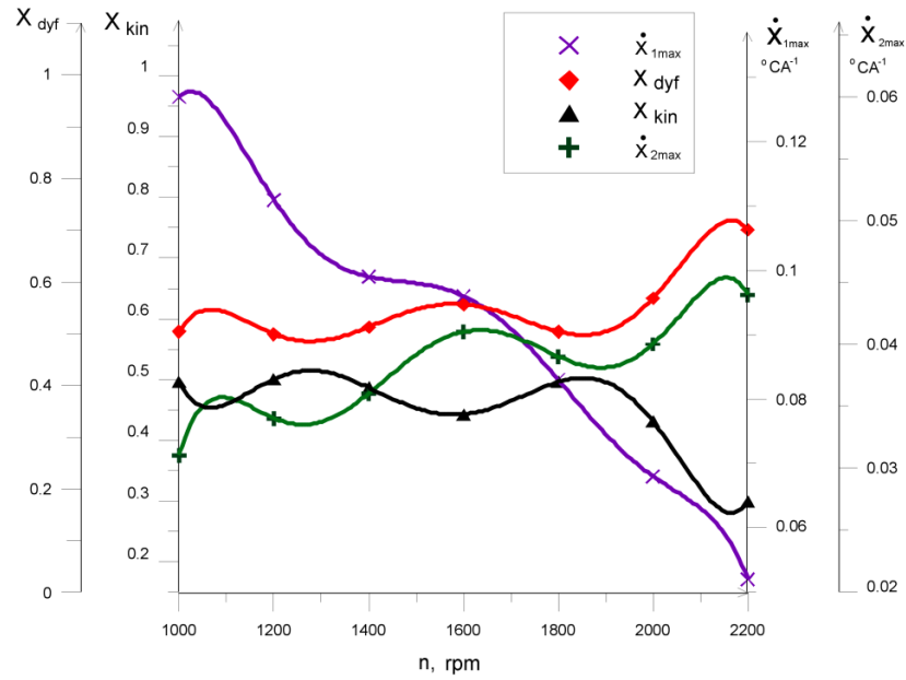
Fig. 8. Combustion process parameters for engine operation according to an external speed characteristic and angle of injection \alpha_{ww} = 17 crankshaft rotation degrees, where: x_{kin} – proportion of kinetic model combustion, x_{dyf} – proportion of diffusion model combustion, \dot{x}_{1max} and \dot{x}_{2max} – first and second maximum heat emission rate
