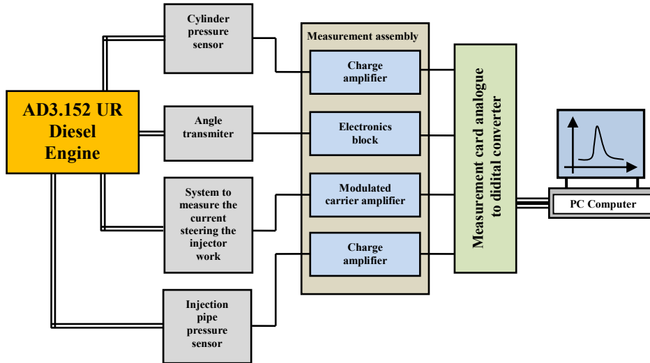
Fig. 2. Flow chart of the piston internal combustion compression - ignition engine rapidly changing parameters measurement system used for the experimental tests
