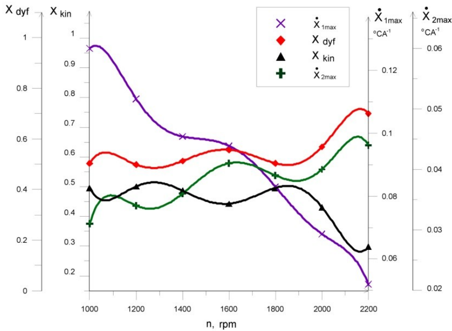
Fig. 7. Combustion process parameters for engine operation according to an external speed characteristic and angle of injection \alpha_{ww} = 13 crankshaft rotation degrees, where: x_{kin} – proportion of kinetic model combustion, x_{dyf} – proportion of diffusion model combustion, \dot{x}_{1max} and \dot{x}_{2max} – first and second maximum heat emission rate
