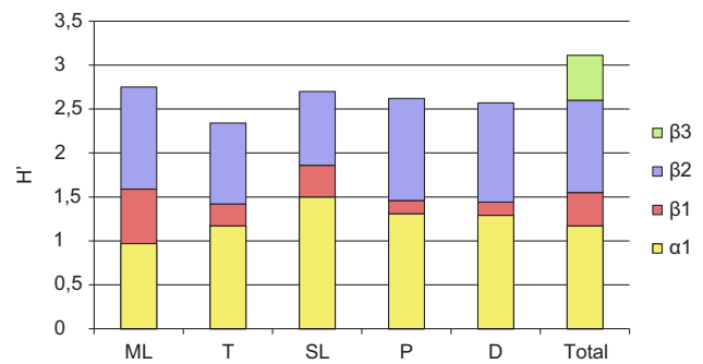
Fig. 5. Shannon entropy partitioning in five habitat types: main Liwiec River channel (ML), tributaries (T), secondary channels of Liwiec (SL), ponds (P) and ditches (D) and in the entire study area (Total); \alpha_1 – mean per sample diversity, \beta_1 – between sample diversity, \beta_2 – between site diversity, \beta_3 – between habitat type diversity
