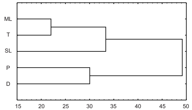
Fig. 3. Dendrogram showing distances among malacofaunas of five habitat types: main Liwec River channel (ML), tributaries (T), secondary channels of Liwec (SL), ponds (P) and ditches (D); cluster analysis based on relative abundance of mollusc species
