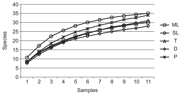
Fig. 2. Sample-based rarefaction curves of mollusc species richness for five habitat types: main Liwec River channel (ML), tributaries (T), secondary channels of Liwec (SL), ponds (P) and ditches (D); (n=11)
