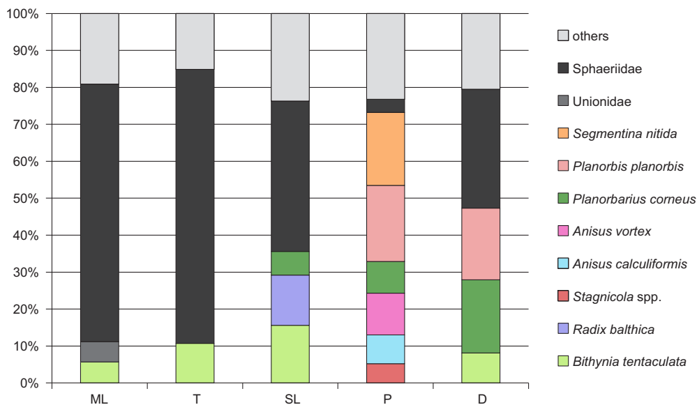
Fig. 4. Dominance patterns of mollusc assemblages in five habitat types: main Liwec River channel (ML), tributaries (T), secondary channels of Liwec (SL), ponds (P) and ditches (D)
