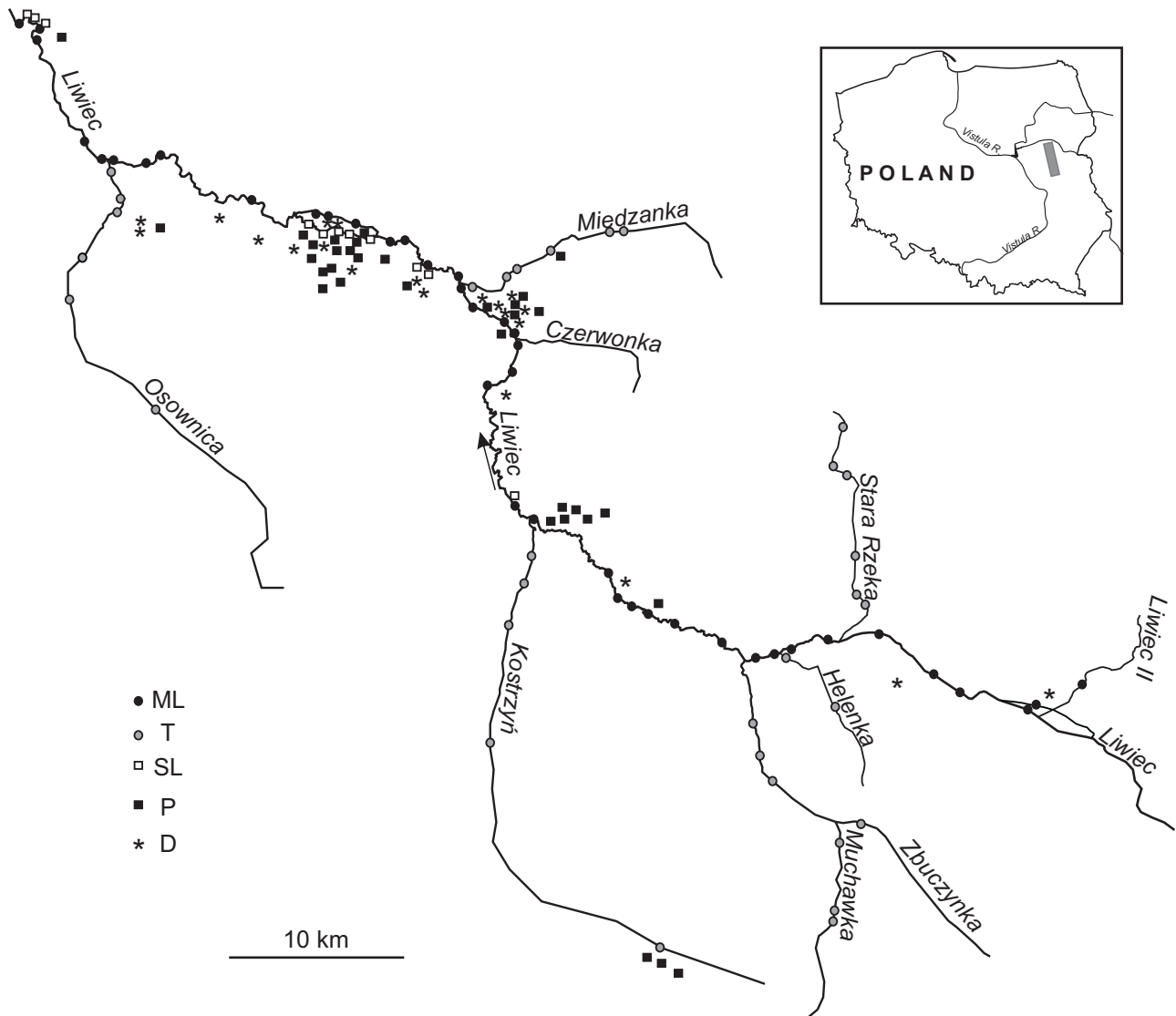
Fig. 1. Study area and location of the investigated sites; ML – main Liwiec River channel, T – tributaries, SL – secondary channels of Liwiec, P – ponds, D – ditches; grey rectangle – location of the study area on the map of Poland
