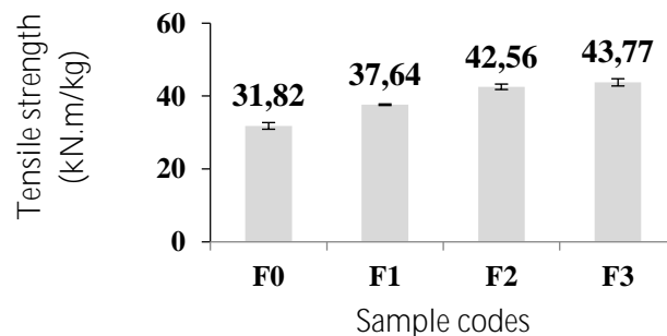
Fig. 3. Change in tensile strength of base paper and sized papers
