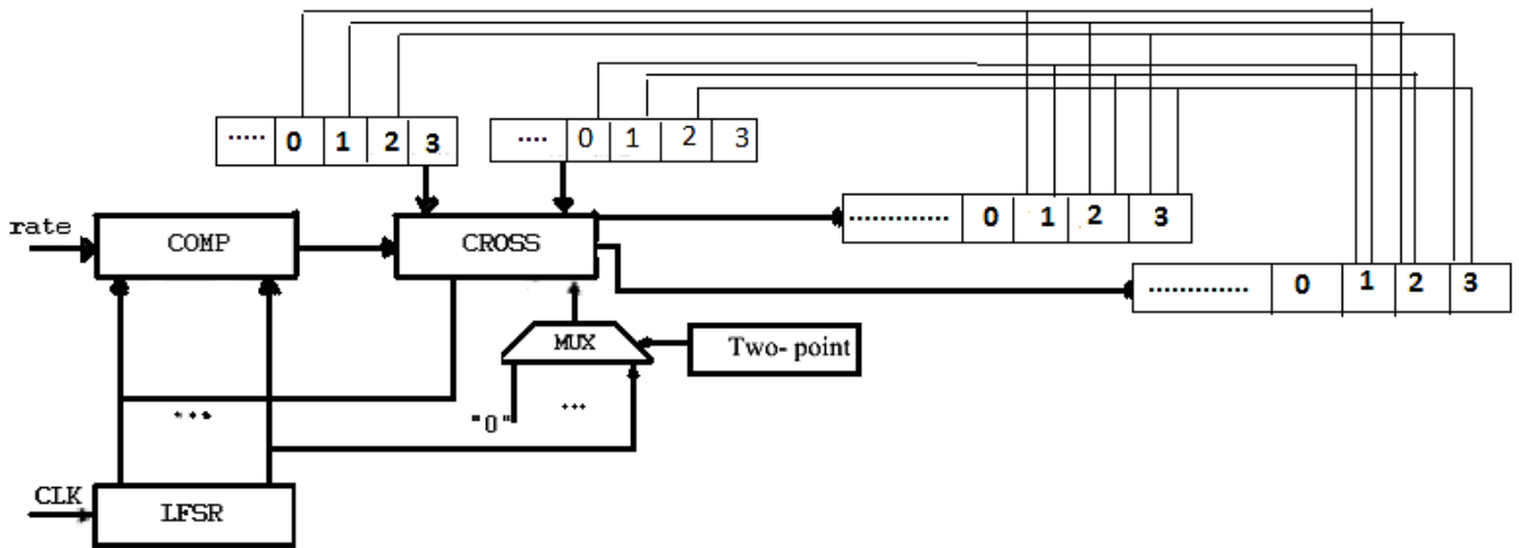
Figure 6. Hardware of crossover operator.
