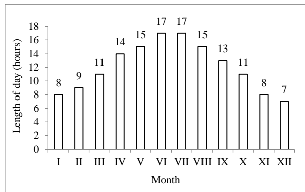
Fig. 1. Average length of day in Poland (Kalda & Smorağ 2012)
