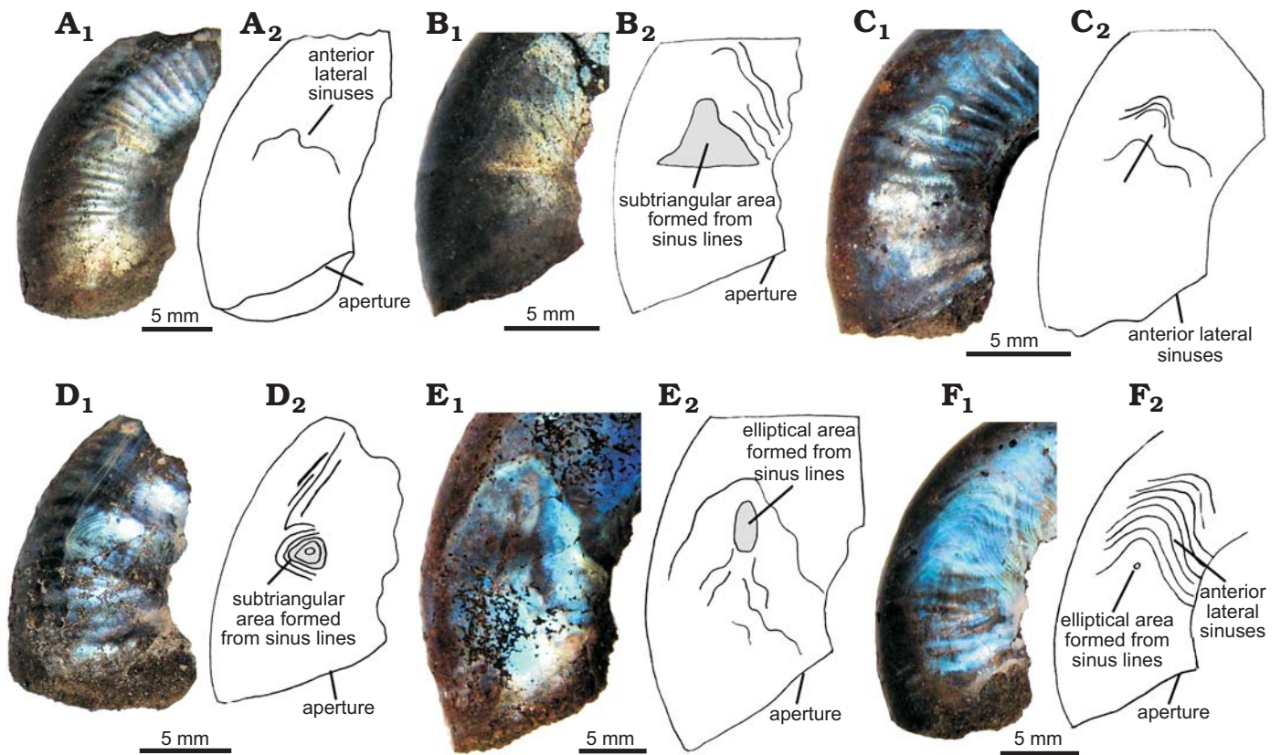
Fig. 11. Apertural parts of the anterior lateral sinuses of Kachpurites fulgens (Trautschold, 1861) from Late Volgian ( Kachpurites fulgens Zone), Moscow region, Eganovo locality (B) and Mnevniki locality (A, C–F). A. MSU 113/24, lateral sinus line in the apertural part of the body chamber. B. MSU 113/7 (see also Fig. 6B), apertural part of the body chamber with lateral sinuses. C. MSU 113/12 (see also Fig. 10B), lateral sinuses in the apertural part of the body chamber. D. MSU 113/23, apertural part of the body chamber with lateral sinuses. E. MSU 113/27, apertural part of the body chamber with a very bright lateral sinus. F. MSU 113/6 (see also Fig. 10C), apertural part of the body chamber. Apertural edge is not preserved. Photographs (A 1 –F 1 ) and explanatory drawings (A 2 –F 2 ).
