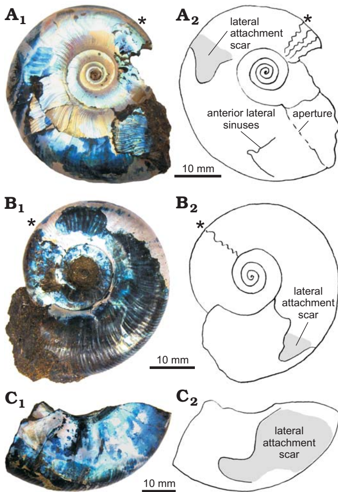
Fig. 5. Lateral attachment structures on Kachpurites chermukhensis Mitta, Michailova, and Sumin 1999 shells from Late Volgian ( Kachpurites fulgens Zone), Yaroslavl region, Chermukha locality. A. MSU 113/3, whole shell with a scar at the middle section of the body chamber and a lateral sinus, which is located ventro-laterally not far from the aperture. B. MSU 113/10, shell with the apertural part of the body chamber not preserved, the scars are slightly asymmetric. C. MSU 113/36, fragment of the body chamber of ribbed macroconch, with scars on both sides of the shell. The scar demonstrate ventro-lateral projection on its front part. Asterisks mark the base of the body chamber. Photographs (A 1 –C 1 ) and explanatory drawings (A 2 –C 2 ).
