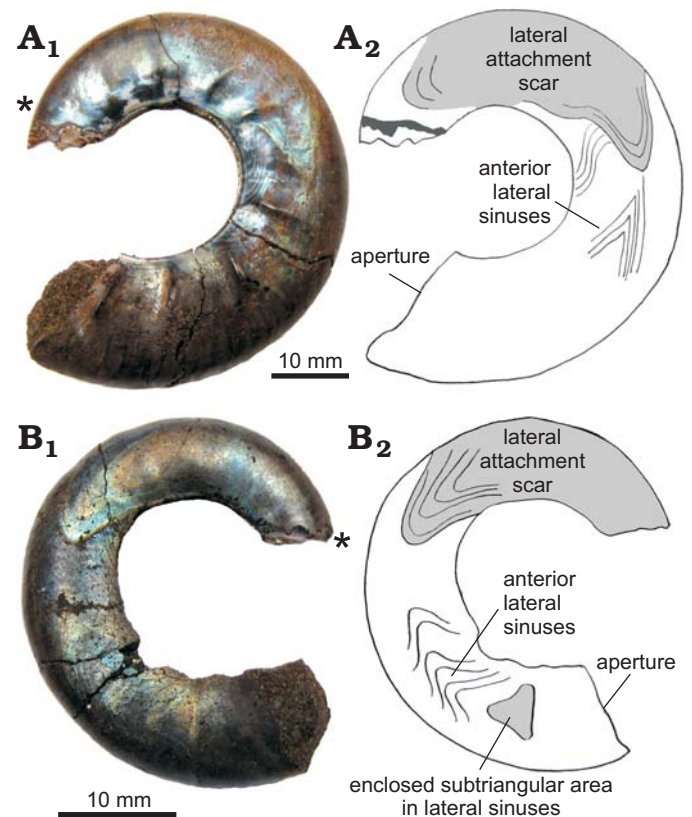
Fig. 6. Lateral attachment scars and lateral sinuses on Kachpurites fulgens (Trautschold, 1861) shells from Late Volgian ( Kachpurites fulgens Zone), Moscow region, Mnevniky locality (A), and Eganovo locality (B). A. MSU 113/1, fully preserved body chamber. Bright scars and lateral sinuses on both sides of the shell. Posterior parts of the scars visible near the last septum. B. MSU 113/7, complete body chamber with scars and lateral sinuses. It is clearly visible that lateral sinuses are located at a distance from the aperture. Asterisks mark the base of the body chamber. Photographs (A 1 , B 1 ) and explanatory drawings (A 2 , B 2 ).
