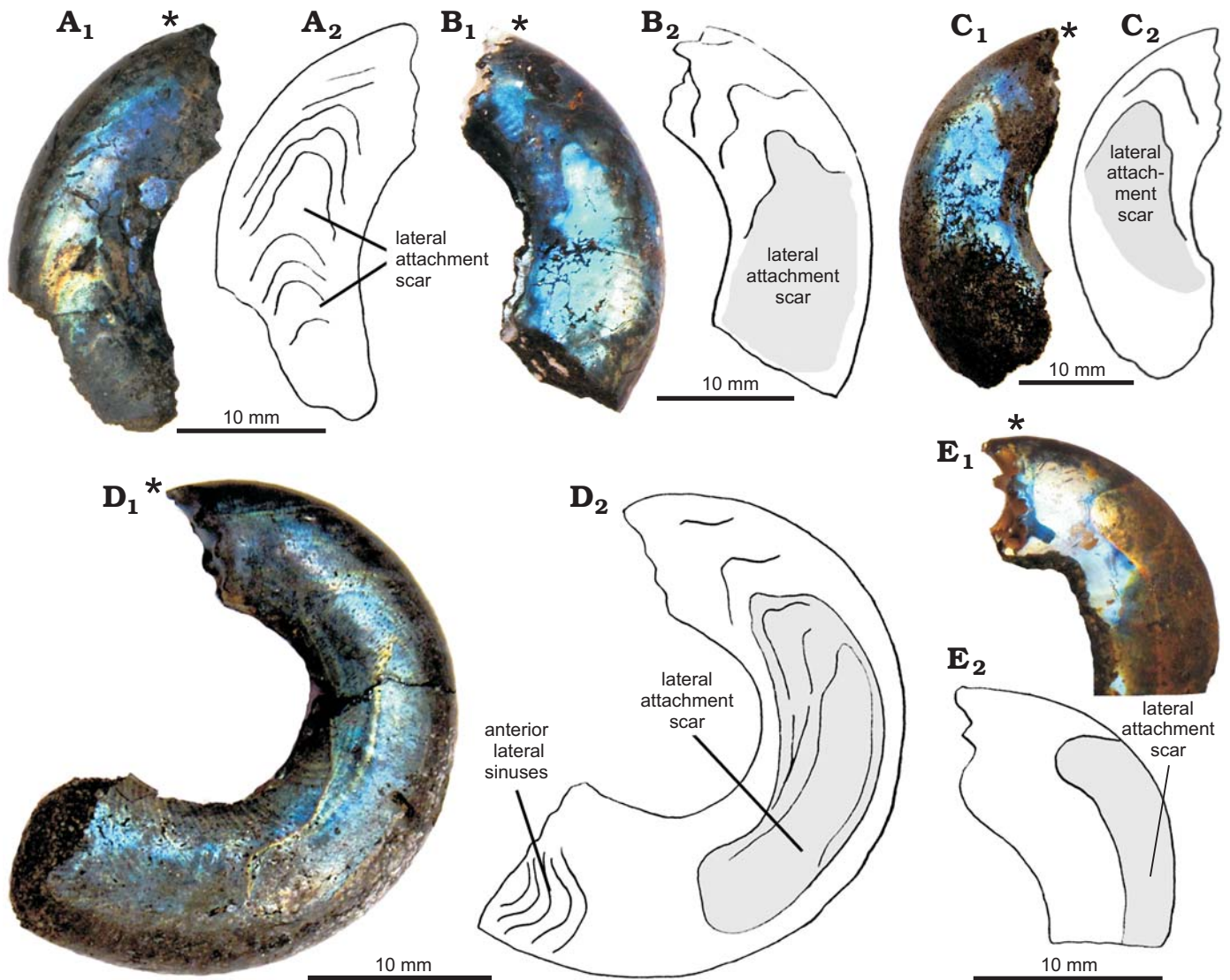
Fig. 9. Posterior borders of the lateral attachment scars on the Kachpurites fulgens (Trautschold, 1861) (A–D) and Garniericeras catenulatum (Fischer, 1830) (E) shells from Late Volgian ( Kachpurites fulgens and Craspedites subditus zones, respectively), Moscow region, Eganovo locality (A–D), Kuntsevo locality (E). A. MSU 113/29, apical part of body chamber with a series of posterior borders of scars very similar to the lateral sinuses. B. MSU 113/32, sinus-like lines on the posterior part of the shell, scars near the last septum. C. MSU 113/33, sinus-like lines on the posterior part of the shell, scars near the last septum. D. MSU 113/8, part of body chamber with scars and lateral sinuses. Scar has a series of clearly visible sinus-like posterior borders. The specimen is preserved without aperture. E. MSU 113/43, apical part of the body chamber, posterior border of a scar is visible on one side of this specimen at a distance from the last septum. Asterisks mark the base of the body chamber. Photographs (A 1 –E 1 ) and explanatory drawings (A 2 –E 2 ).
