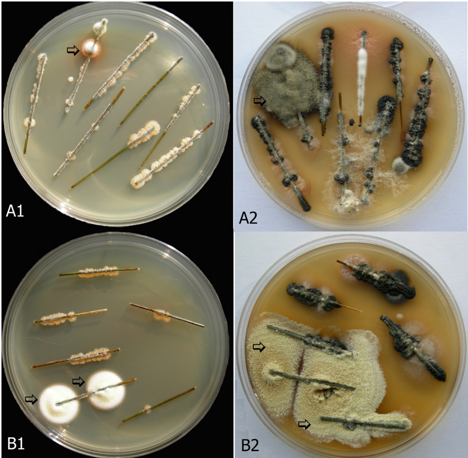
Fig. 1. Aureobasidium pullulans : A 1 – after 10 days; A 2 – after 30 days; Penicillium expansum : B1 – after 10 days; B2 – after 30 days. Both strains were cultivated on Ferency medium.
