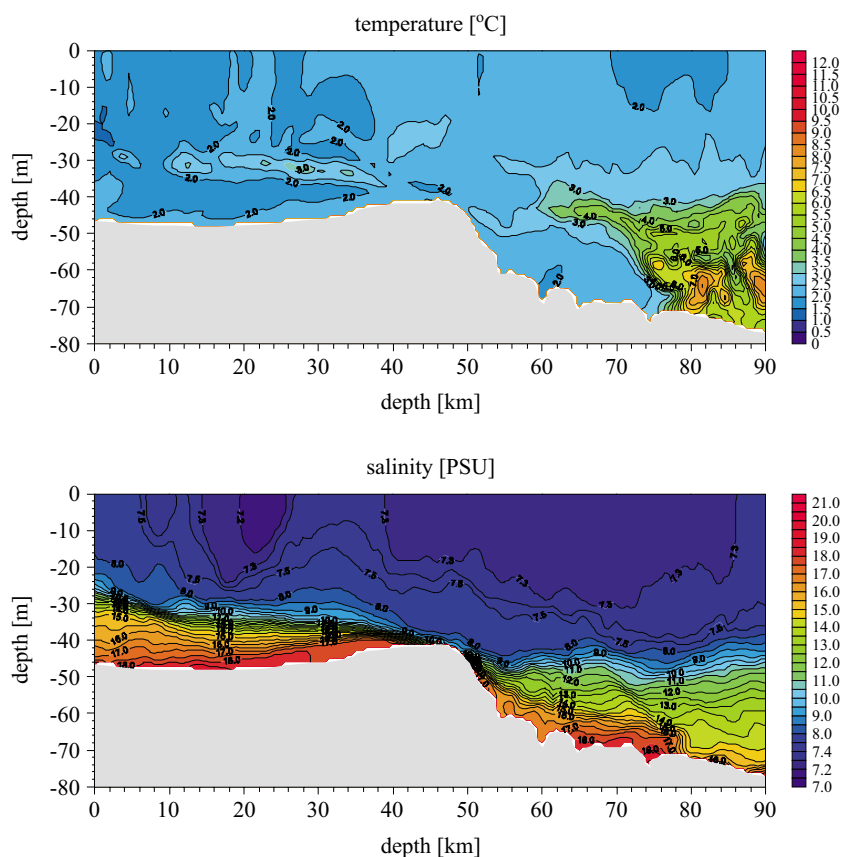
Fig. 6. Temperature and salinity in the Bornholm Gate. 7 February 2003
