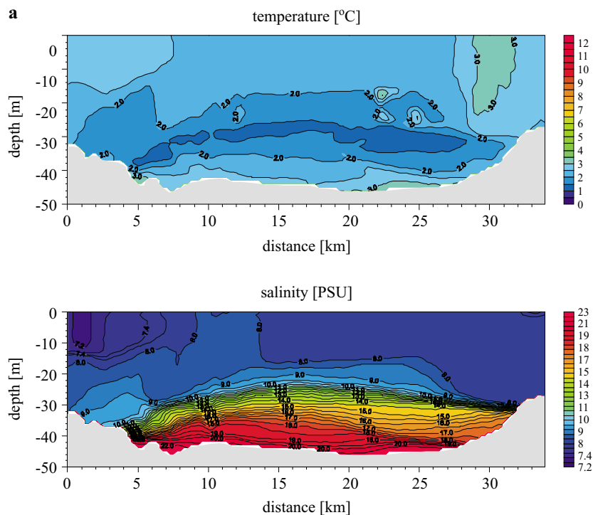
Fig. 3. Temperature, salinity and currents. 25–26 January 2003. Arkona Basin (a) and Bornholm Gate (b)
