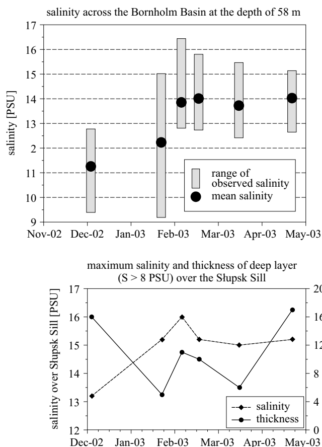
Fig. 18. Transport of the inflow waters over the Słupsk Sill
