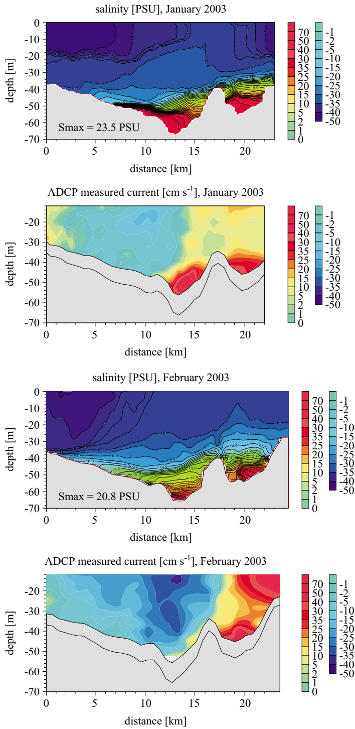
Fig. 15. Transportation of the inflow waters through the Bornholm Channel
