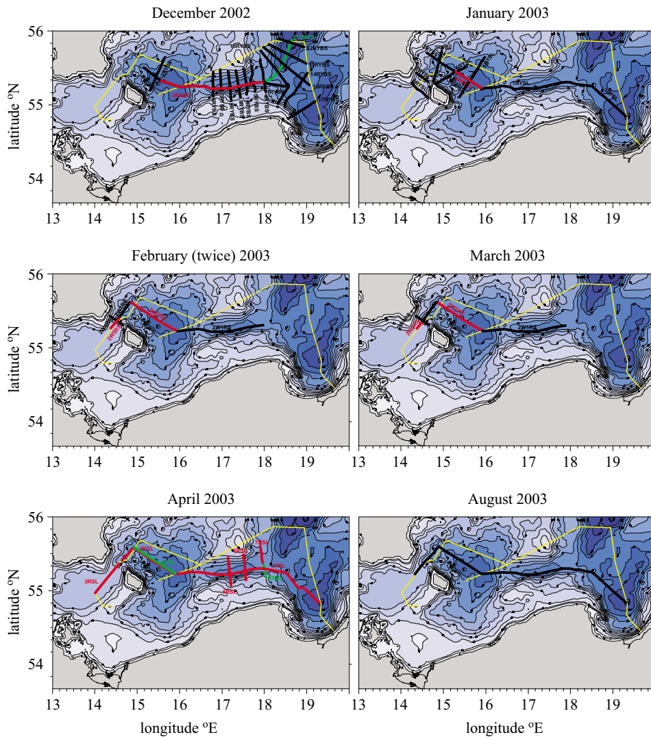
Fig. 1. Maps of investigations during the main inflow in winter, spring and summer 2003
