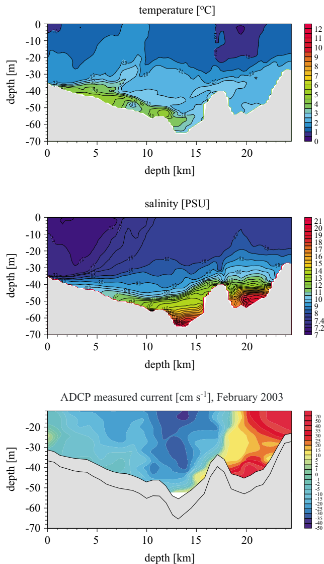
Fig. 9. Temperature and salinity across the Bornholm Gate. 16–18 February 2003
