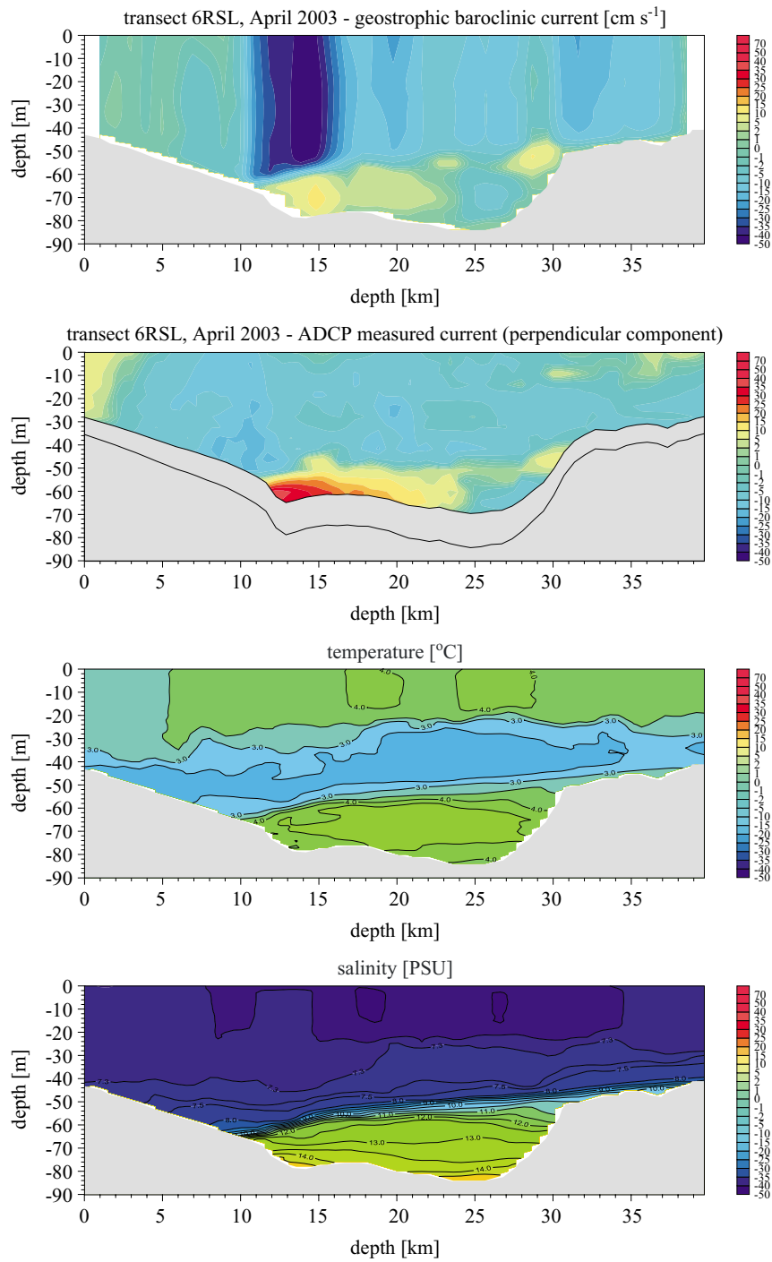
Fig. 20. Transport of the inflow waters in the Slupsk Channel at transect 6RSL. April 2003
