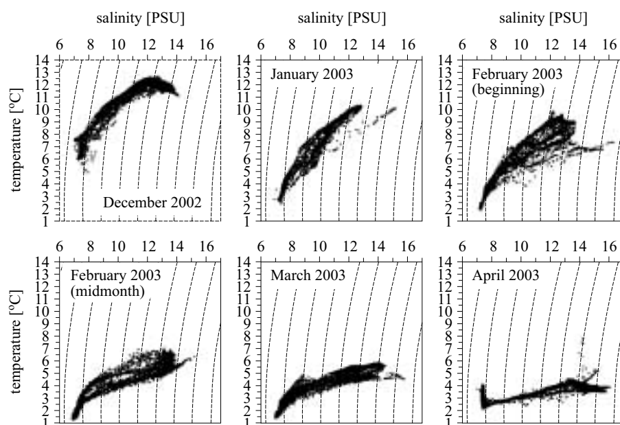
Fig. 22. Transformation of water masses during the successive stages of inflow in 2003 – Ślupsk Channel
