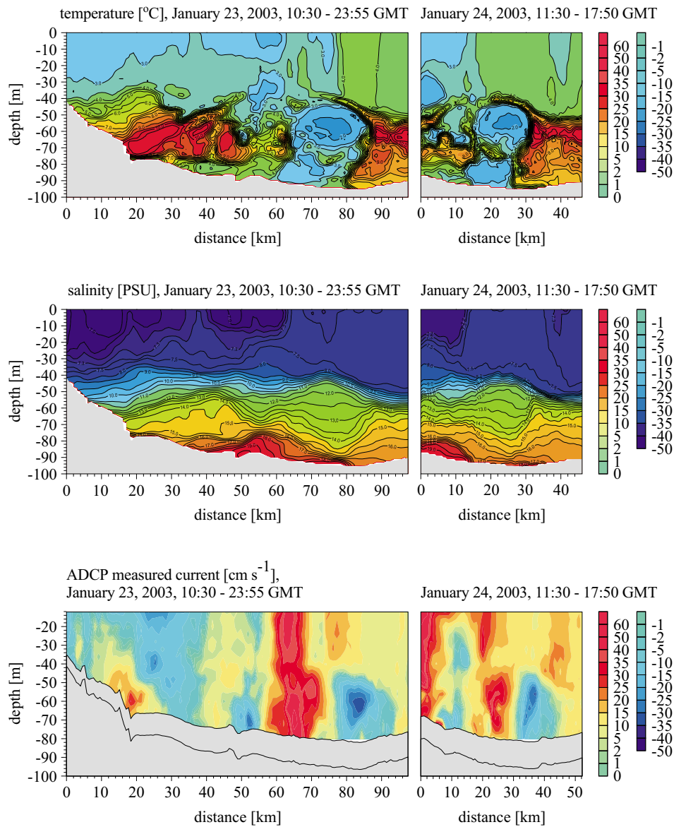
Fig. 17. Eddies and meandering of slope current in the Bornholm Basin. January 2003
