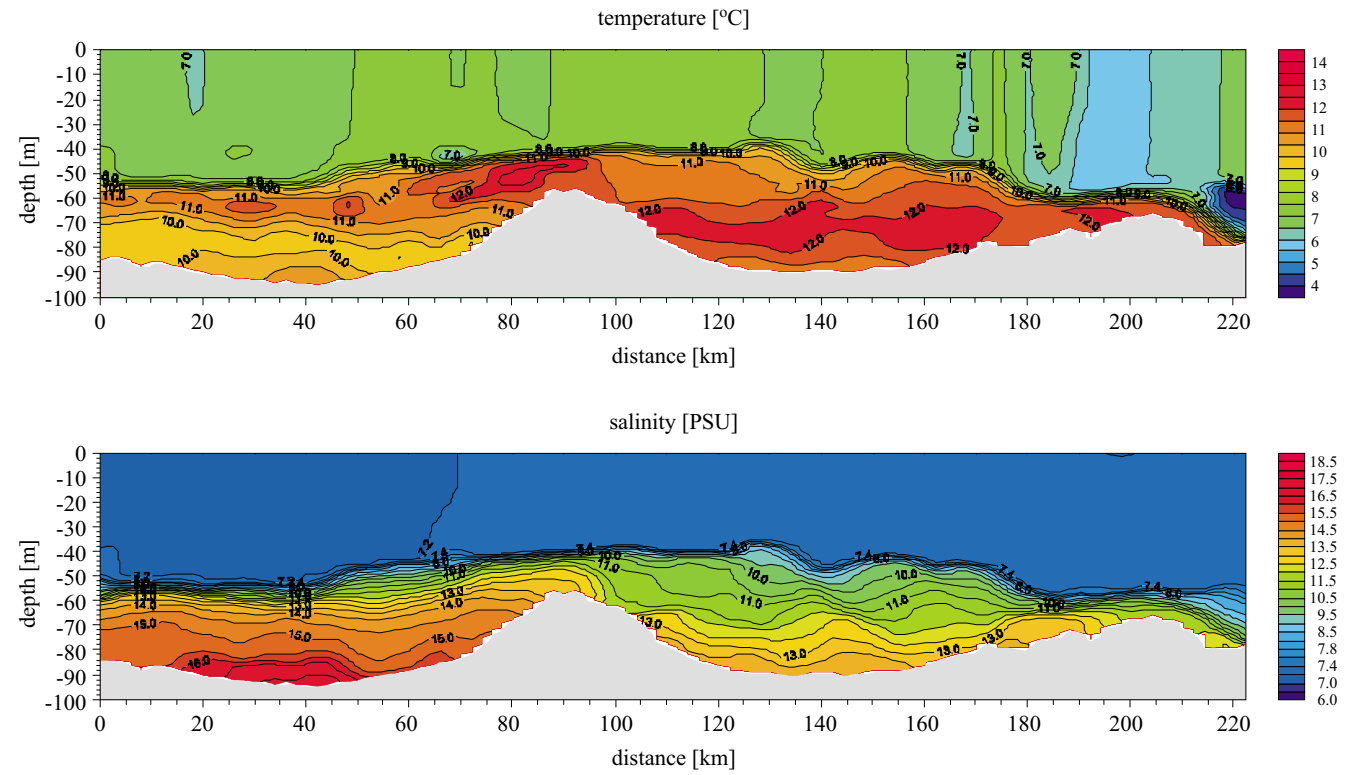
Fig. 2. Temperature and salinity along the main transect. 3–4 December 2002
