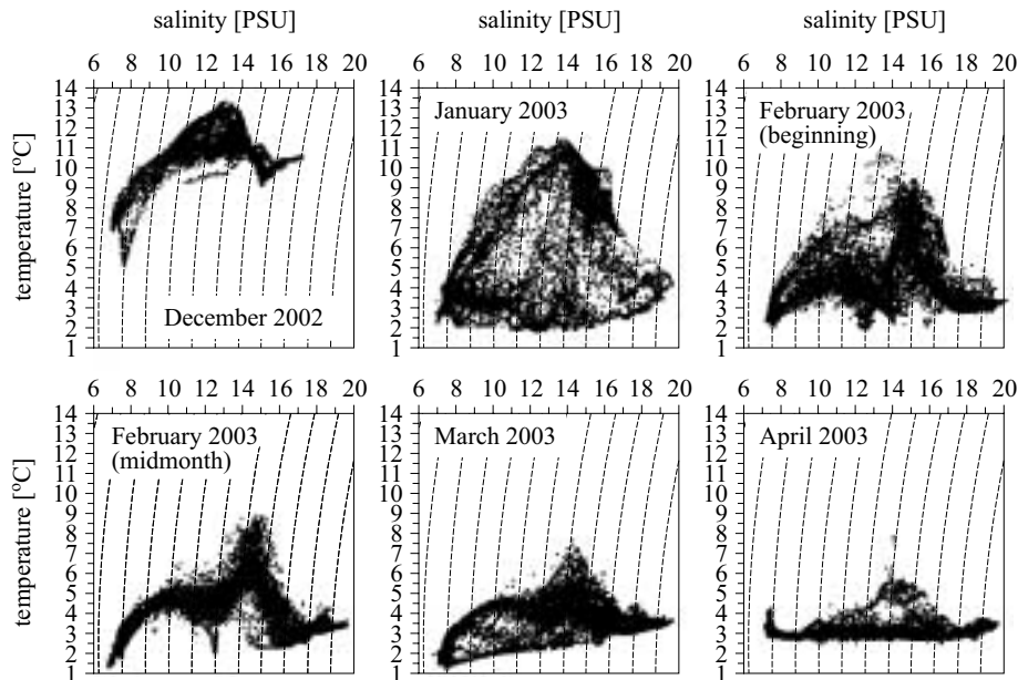
Fig. 21. Transformation of water masses during the successive stages of inflow in 2003 – Bornholm Basin
