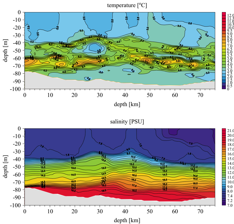
Fig. 8. Temperature and salinity in the Bornholm Deep. 6–7 February 2003
