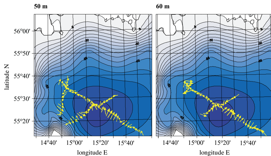
Fig. 5. Currents at the 50 and 60 m levels. ADCP data. January 2003
