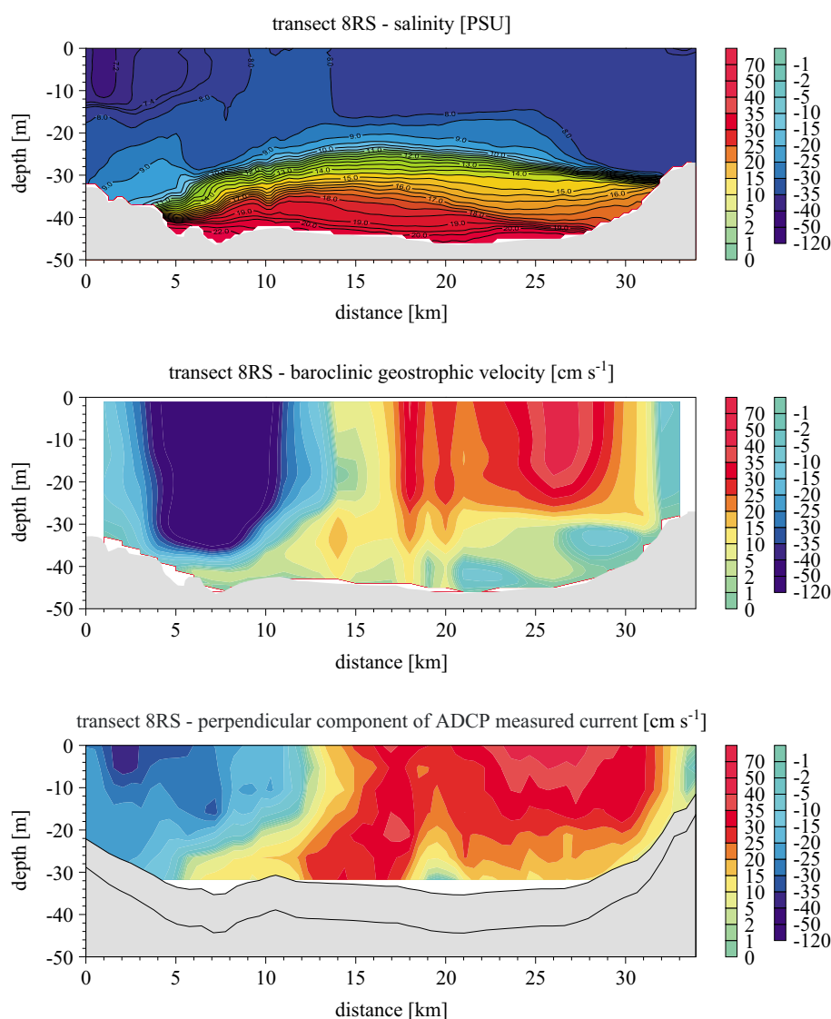
Fig. 14. Pool of the inflow waters in the Arkona Basin. 26 January 2003
