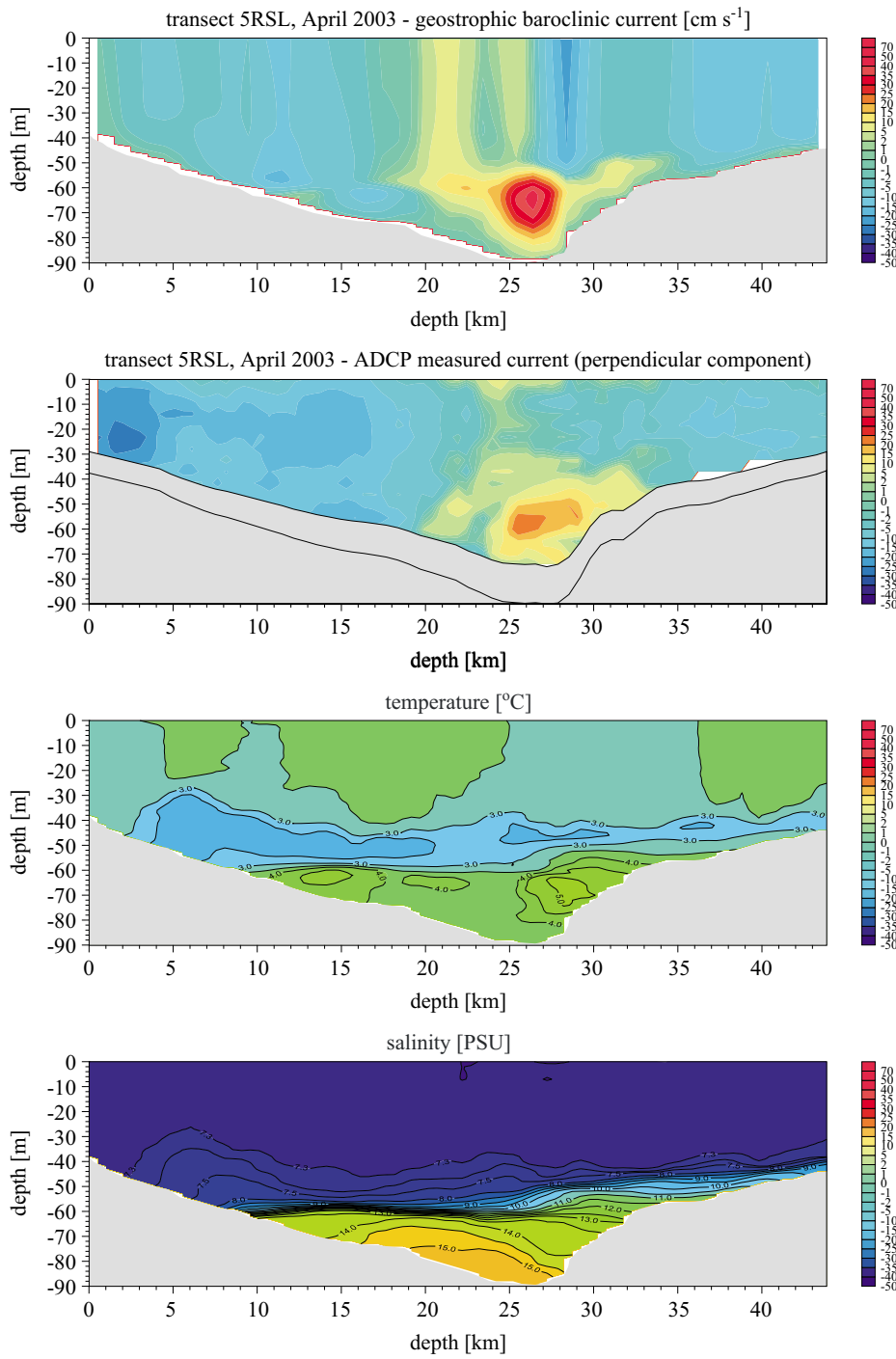
Fig. 19. Transport of the inflow waters in the Ślupsk Channel at transect 5RSL. April 2003
