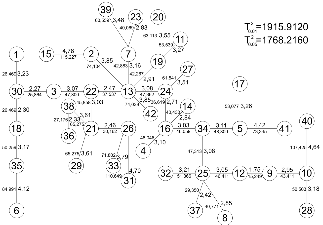
Fig. 3. Dendrite of 42 trees of Pinus uncinata – for each of the shortest Mahalanobis distances (large numerals) counted the values of Hotelling's T^2 statistics (small numerals). T_{0.01}^2 and T_{0.05}^2 – critical values of Hotelling's T^2 statistics (number of trees 1–7 from Vallibierna, 8–17 from Barranco de Vallibierna, 18–27 from St. Maurici, 28–37 from Tossal de l'Orri de Rubio, 38–42 from Sierra del Cadi)
