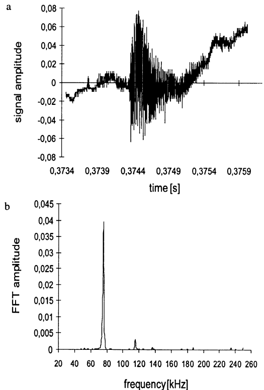
Fig. 2. The characteristics of potato tissue obtained at the strain of -0.2 , and the stress of about 600 kPa. (a) the acoustic emission signal, (b) spectrum analysis of the AE signal by means of FFT.
