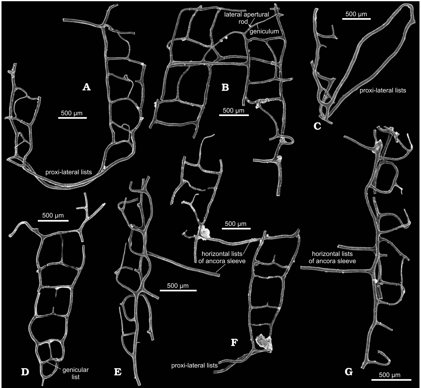
Fig. 3. SEM micrographs of plectograptine retiolitid Kirkgiraptus inexpectans gen. et sp. nov., Neodiversograptus nilssoni Biozone, Ludlow, Poland. A. Rhabdosome with proximal end and two thecal rows, ZPAL G. 40/01, holotype. B. Distal growing end with malformation of the last thecal orifice on the right hand side, ZPAL G. 40/02, paratype. C. Fragment of proximal end with proxi-lateral lists complete, ZPAL G. 40/03, paratype. D. Fragment of one thecal row with proximal end, and with malformation proximal to the first genicular list, view from the inside, ZPAL G. 40/04, paratype. E. One thecal row fragment of rhabdosome with two fragments of horizontal lists of ancora sleeve, lateral view, ZPAL G. 40/05, paratype. F. Fragment of rhabdosome with two rows of thecae, ZPAL G. 40/06, paratype. G. Fragment of rhabdosome with one row of thecae, and three pieces of horizontal lists of ancora sleeve, ZPAL G. 40/07, paratype.
