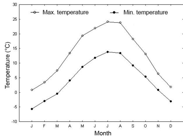
Fig. 2. Mean (1980–2000) minimum and maximum temperatures at the Cz \acute{e} stochowa meteorological station.
