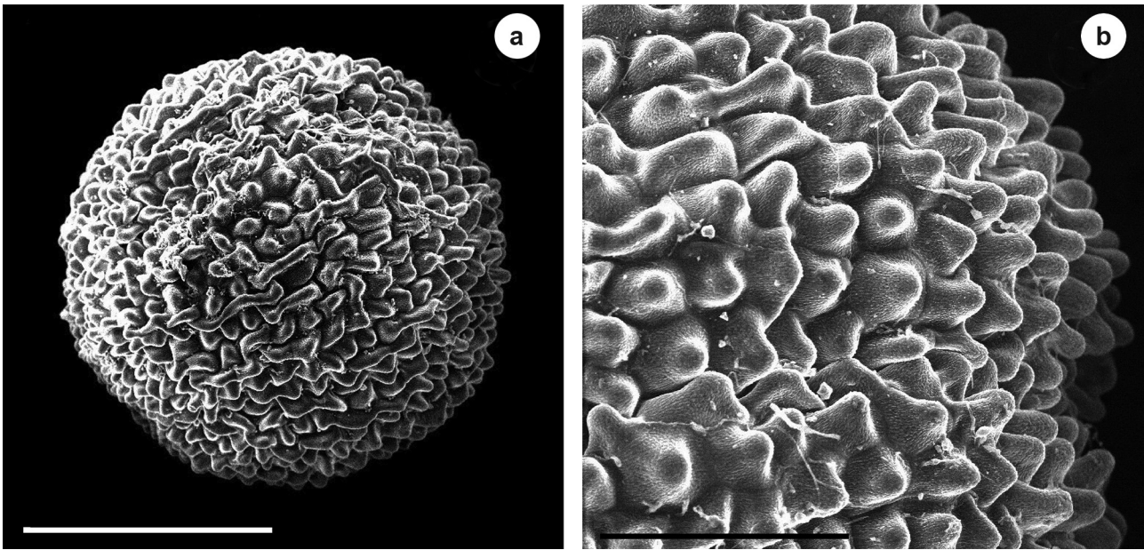
Fig. 1. Scanning electron micrographs of a Galium cracoviense seed. (a) entire mericarp (Bar = 500 \mu\text{m} ), (b) enlargement of mericarp coat (Bar = 200 \mu\text{m} ).
