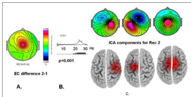
Figure 1. Relative EEG spectra differences between the first and second recordings A. Map of spectra difference (2 rec – 1 rec) at 25 Hz. B. Relative spectra difference (2 rec – 1 re). Below the curve p-values of the spectra difference. Large vertical bars – p < 0.001 , small vertical bars – p < 0.05 . C. Maps and sLORETA images of independent components associated with increase in beta activity.
