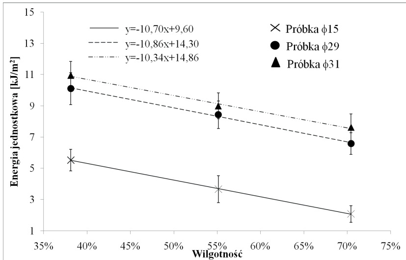
Fig. 9. Comparison of the course of changes of unitary energy (in moisture function) of cutting the Reynoutria sachalinesis’ stem for 3 different diameters
