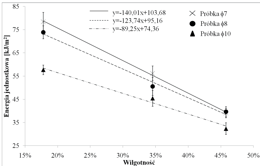
Fig. 8. Comparison of the course of changes of unitary energy (in moisture function) of cutting the Miskanthus ' stem for 3 different diameters
