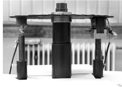
Fig. 2 Laboratory stand for testing circular saws with harmonic method, where: 1 – input function generator, 2 – signal amplifier, 3 – oscilloscope, 4 – inductor, 5 – contactless magneto-inductive sensor
