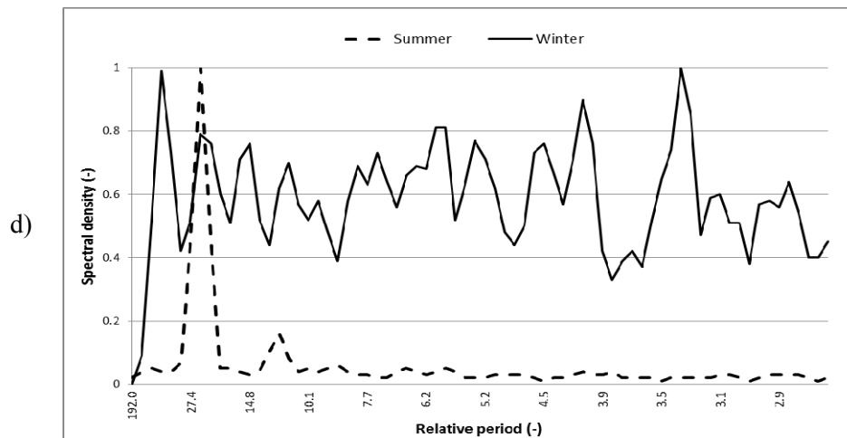
Fig. 4. Estimations of the correlation functions (a, b) and spectral density (c, d) of the stationary random process of T_{soil} diurnal changes at a depth of 10 cm
