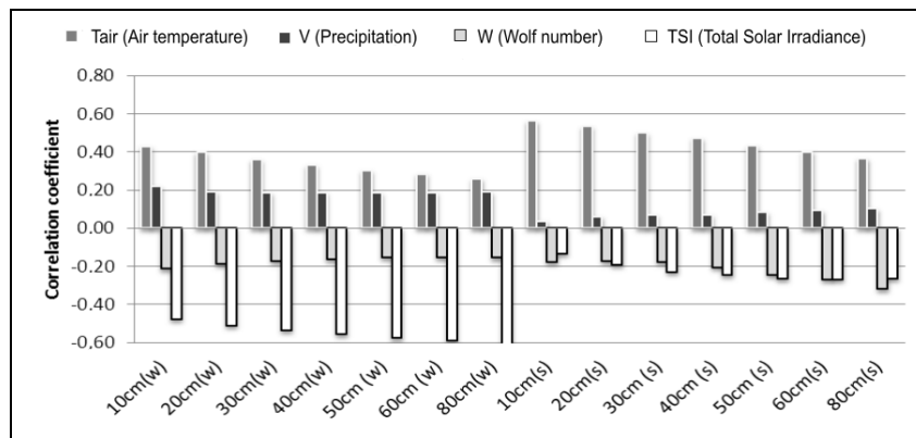
Fig. 12. Correlation coefficients for S02 soil temperature in winter and summer (2009-2010)
