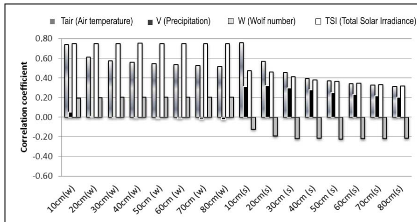
Fig. 14. Correlation coefficients for S04 soil temperature in winter and summer (2011-2012)
