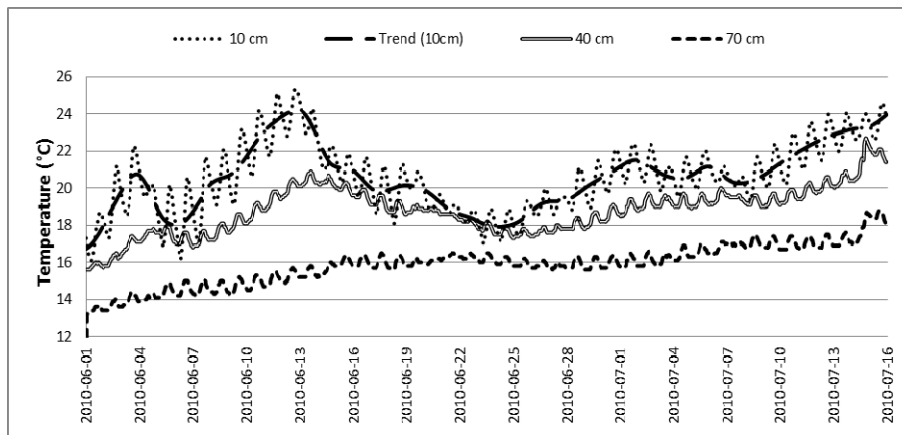
Fig. 3. Temperature time indications at different depths (10, 40, 70 cm) for lowland peat bogs and their low-frequency trend
