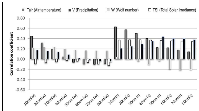
Fig. 13. Correlation coefficients for S03 soil temperature in winter and summer (2010-2011)
