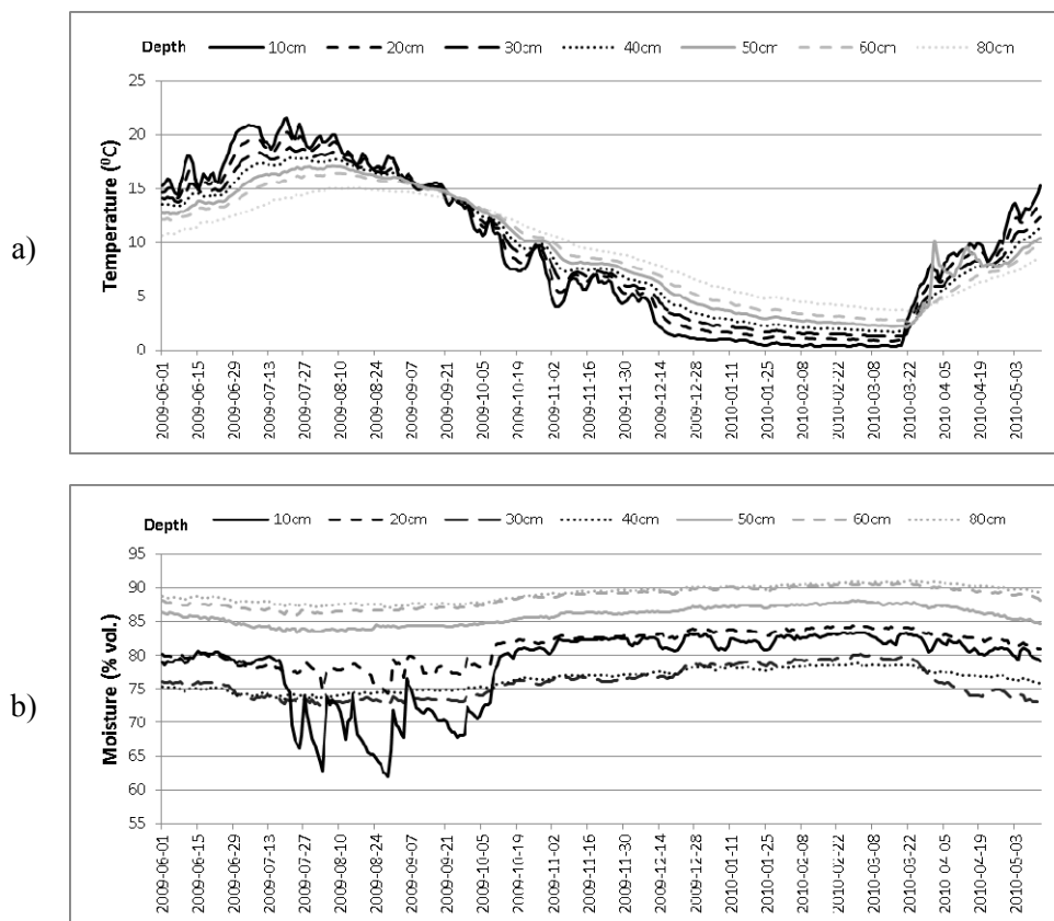
Fig. 8. (a) T_{soil} and (b) \theta_{soil} dynamics for S02 in the years 2009-2010
