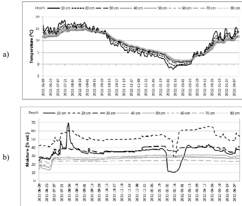
Fig. 10. (a) T_{soil} and (b) \theta_{soil} dynamics for S04 in the years 2011-2012
