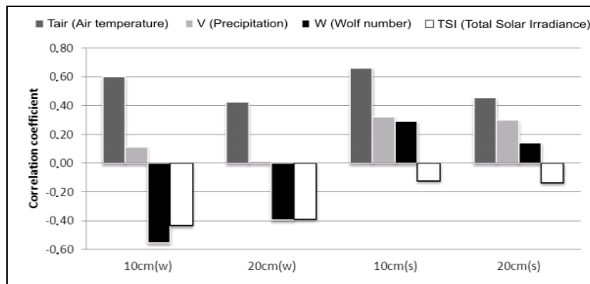
Fig. 11. Correlation coefficients for S01 soil temperature in winter and summer (2008-2009) at depth of 10 cm and 20 cm
