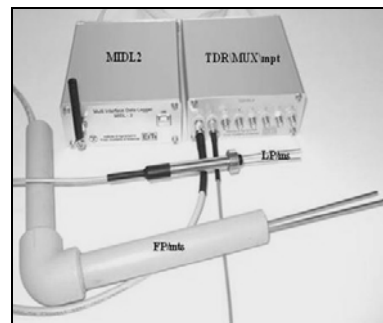
Fig. 2. TDR/MUX/mts ecosystem monitoring network
