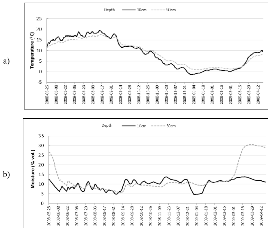
Fig. 7. (a) T_{soil} and (b) \theta_{soil} dynamics for S01 in the years 2008-2009
