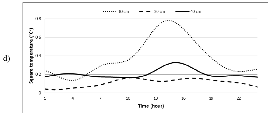
Fig. 5. Estimations of mathematical expectation (a, b) and dispersion (c, d) correlated process of soil temperature diurnal variations in summer at depths: 10 cm, 20 cm and 40 cm
