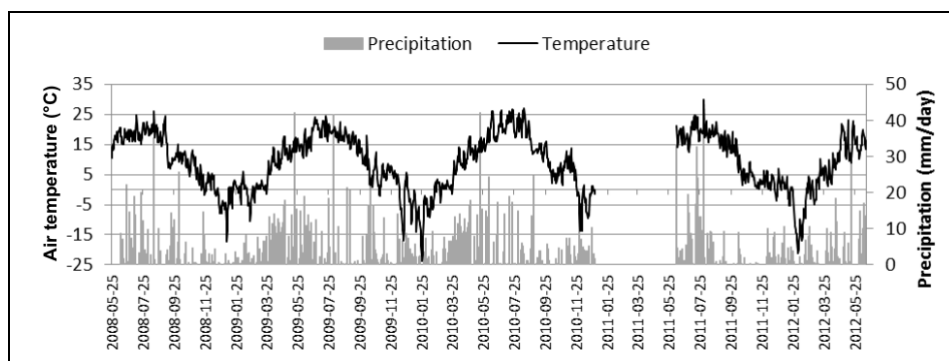
Fig. 6. Dynamics of climate parameters at the Shatsk National Natural Park during the years 2008-2012
