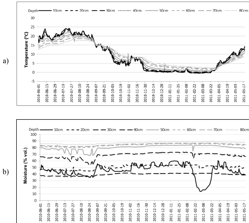
Fig. 9. (a) T_{soil} and (b) \theta_{soil} dynamics for S03 in the years 2010-2011
