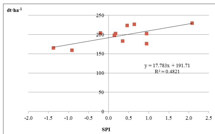
Figure 2. The relationship between the tuber yield of potato (dt·ha -1 ) in the period 1999-2010 in the region of Kujawsko-Pomorskie and the value of SPI during July-August
